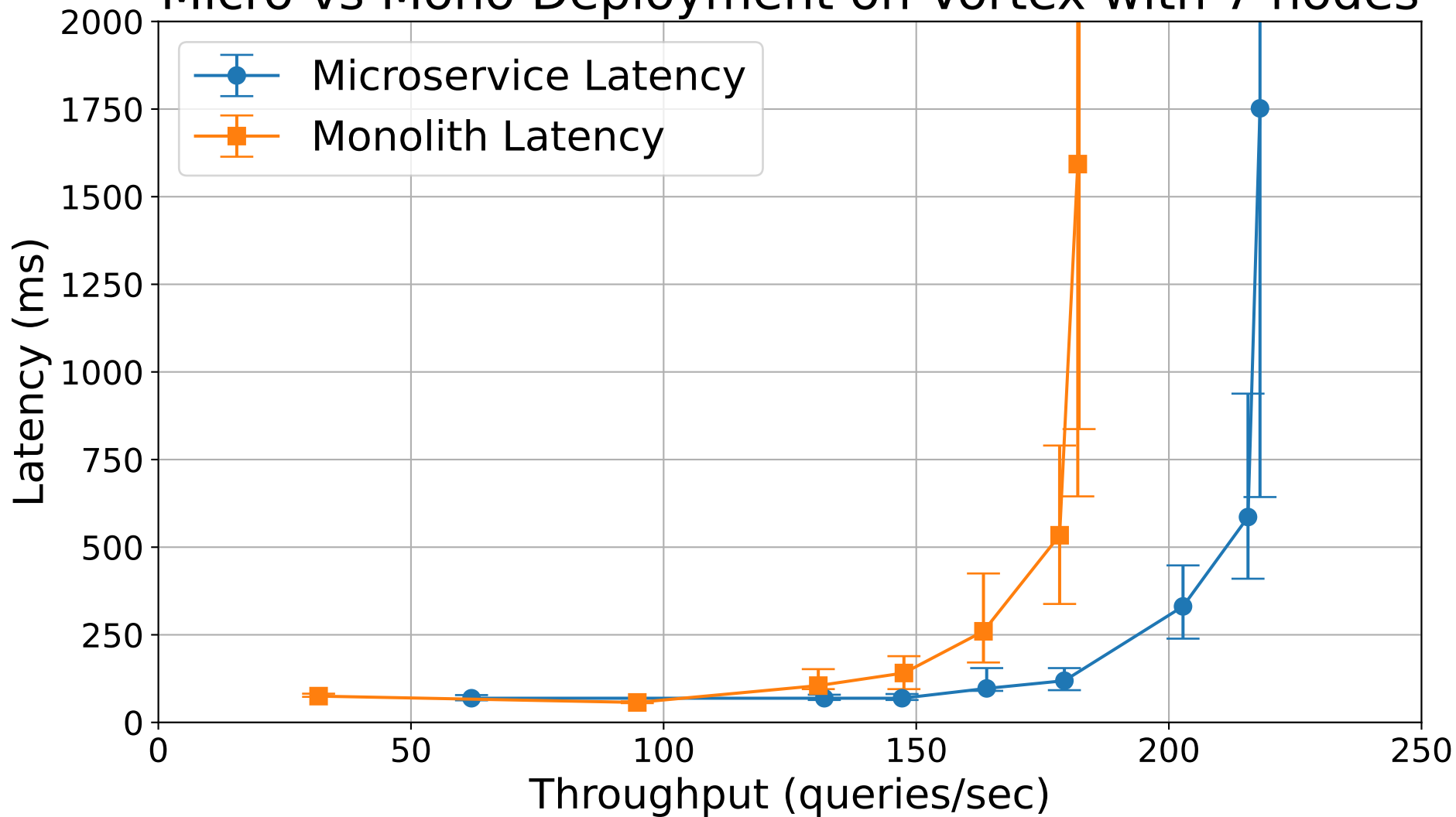
Micro vs Mono Deployment on Vortex with 7 nodes
