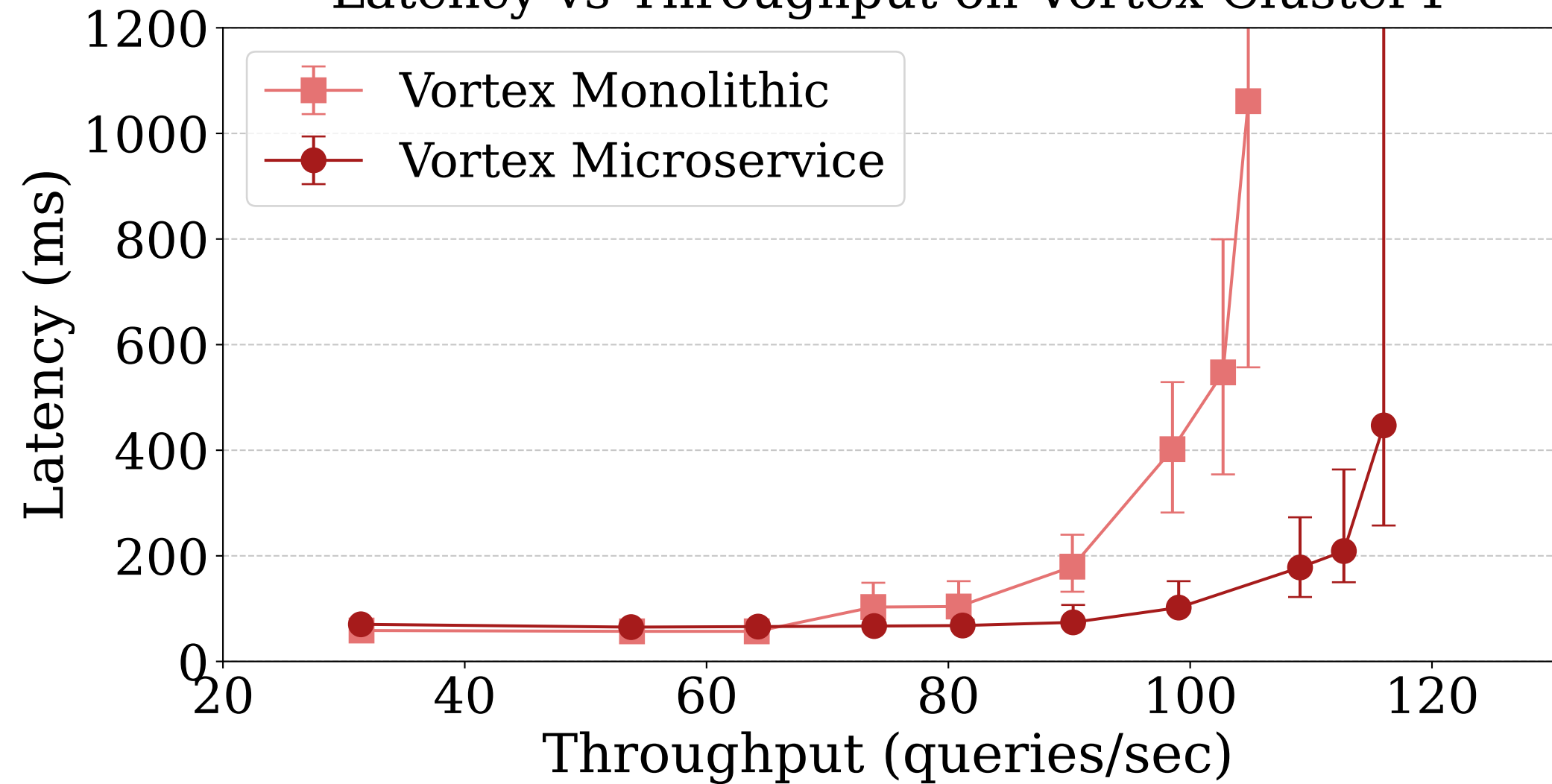
Latency vs Throughput on Vortex Cluster4
