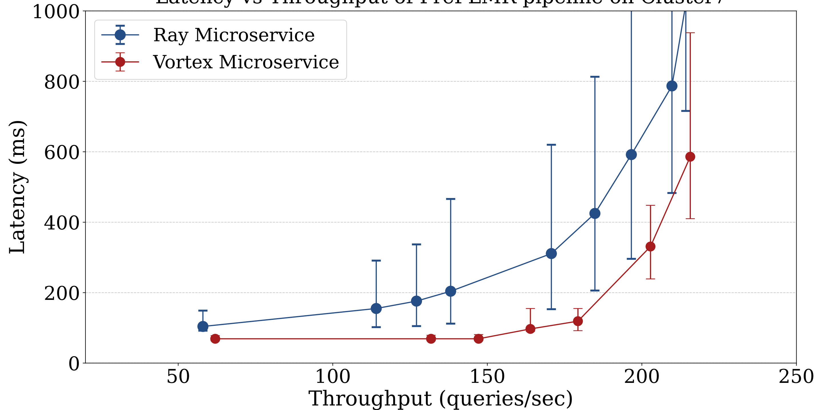
Latency vs Throughput of PreFLMR pipeline on Cluster7
