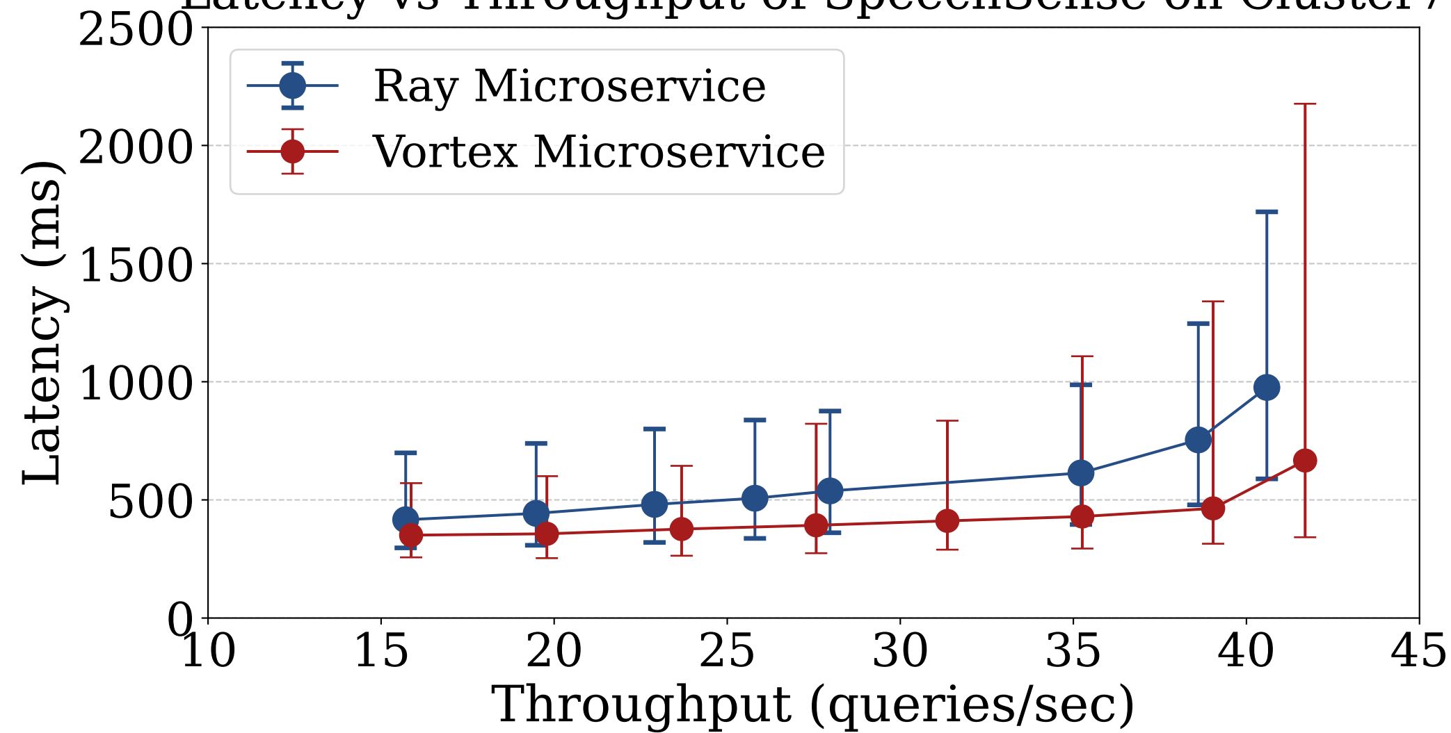
Latency vs Throughput of SpeechSense on Cluster7
