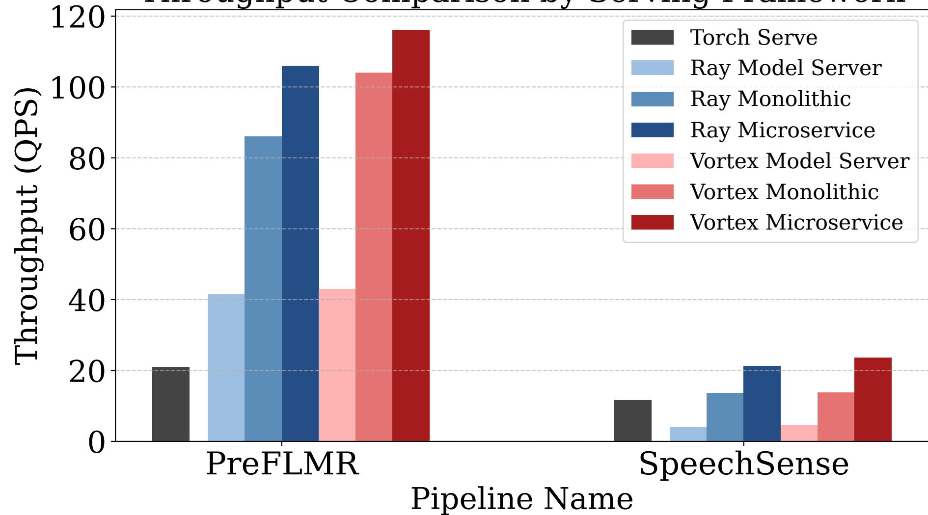
Throughput Comparison by Serving Framework
