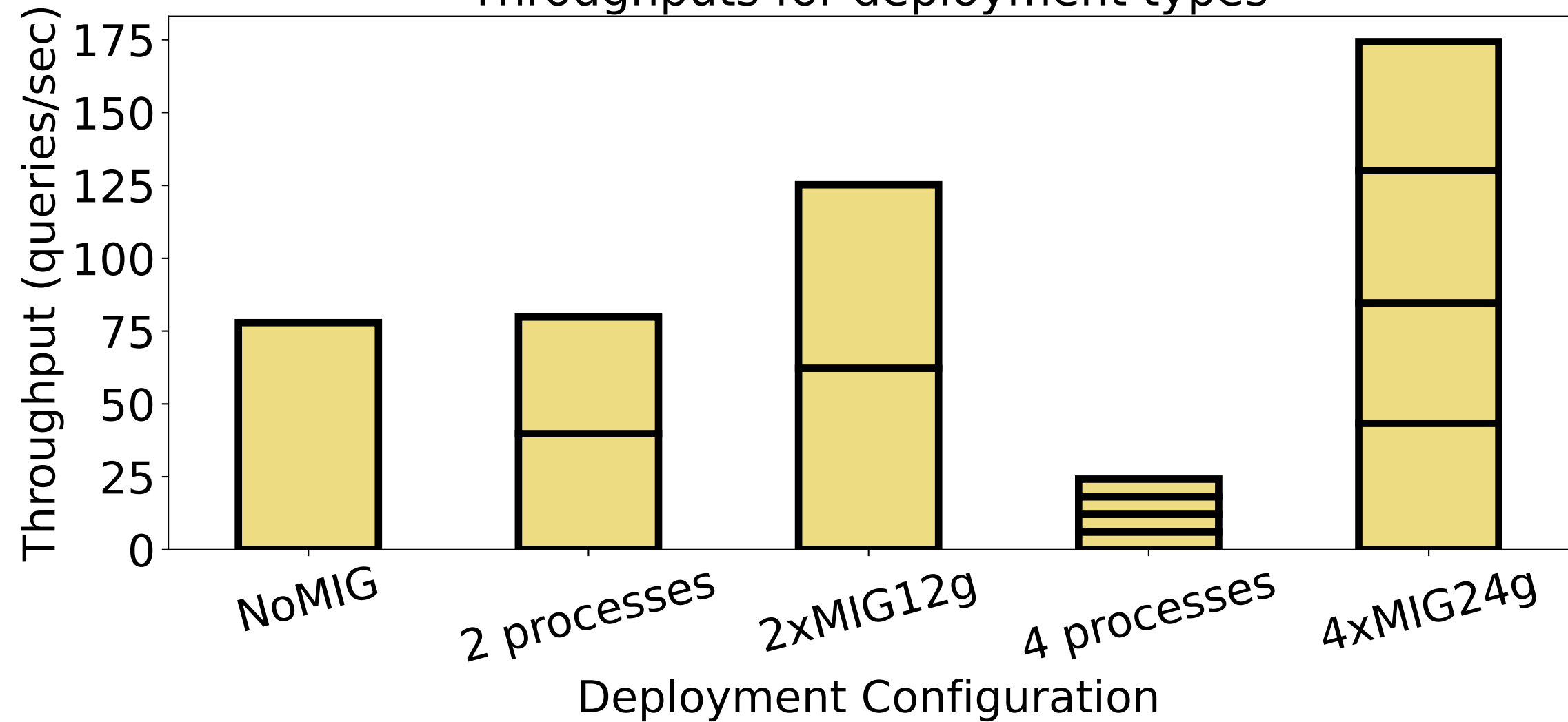
Throughputs for deployment types
