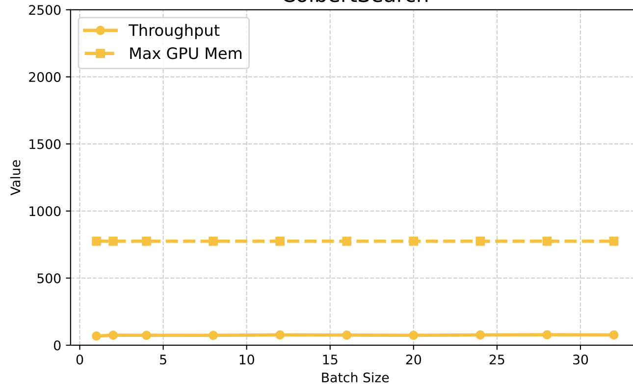
ColbertSearch
