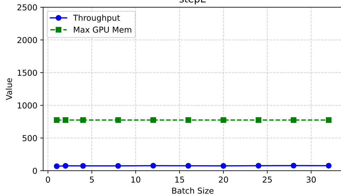
stepE
