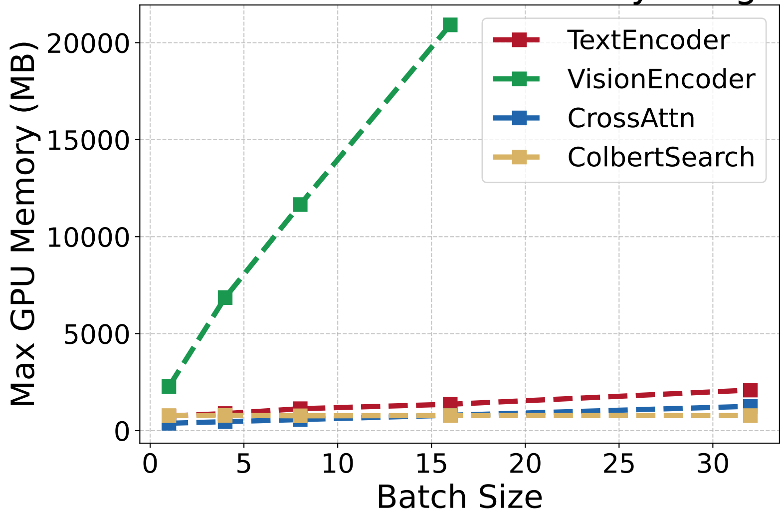
Batch Size vs. GPU Memory Usage
