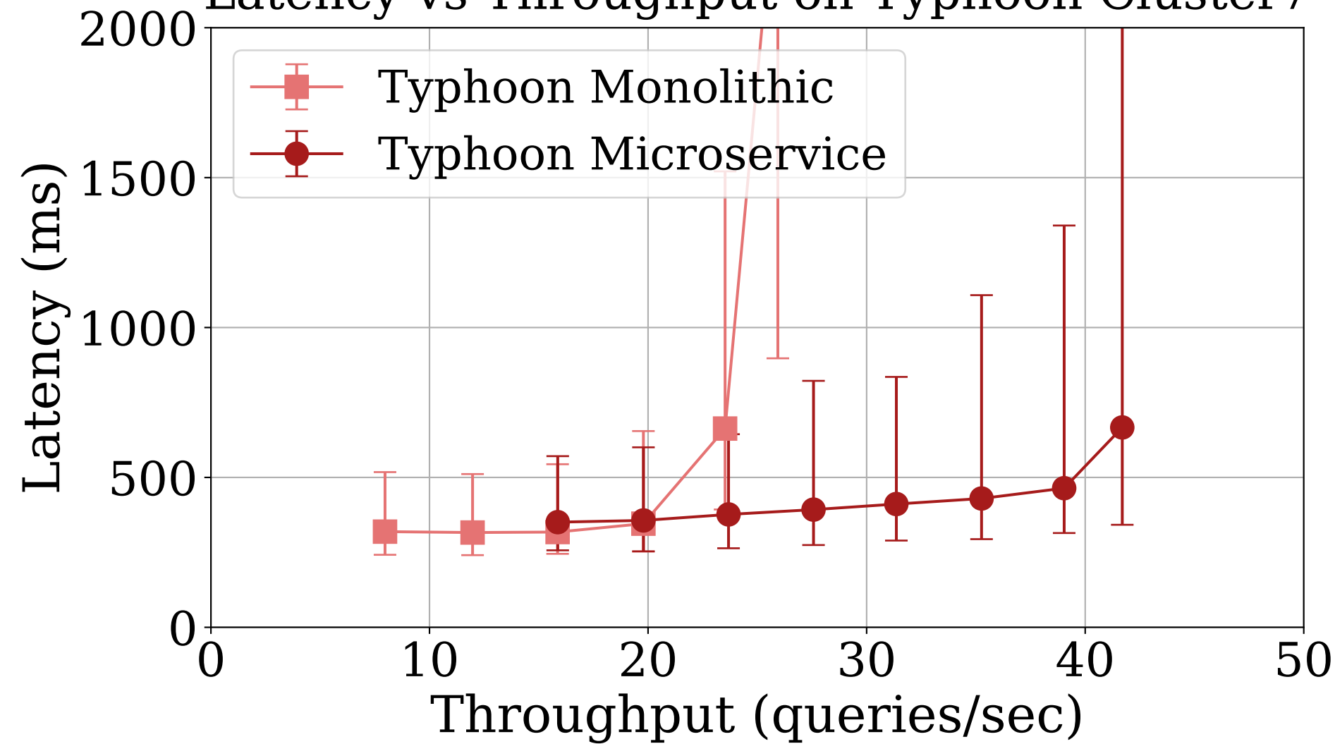
Latency vs Throughput on Typhoon Cluster7
