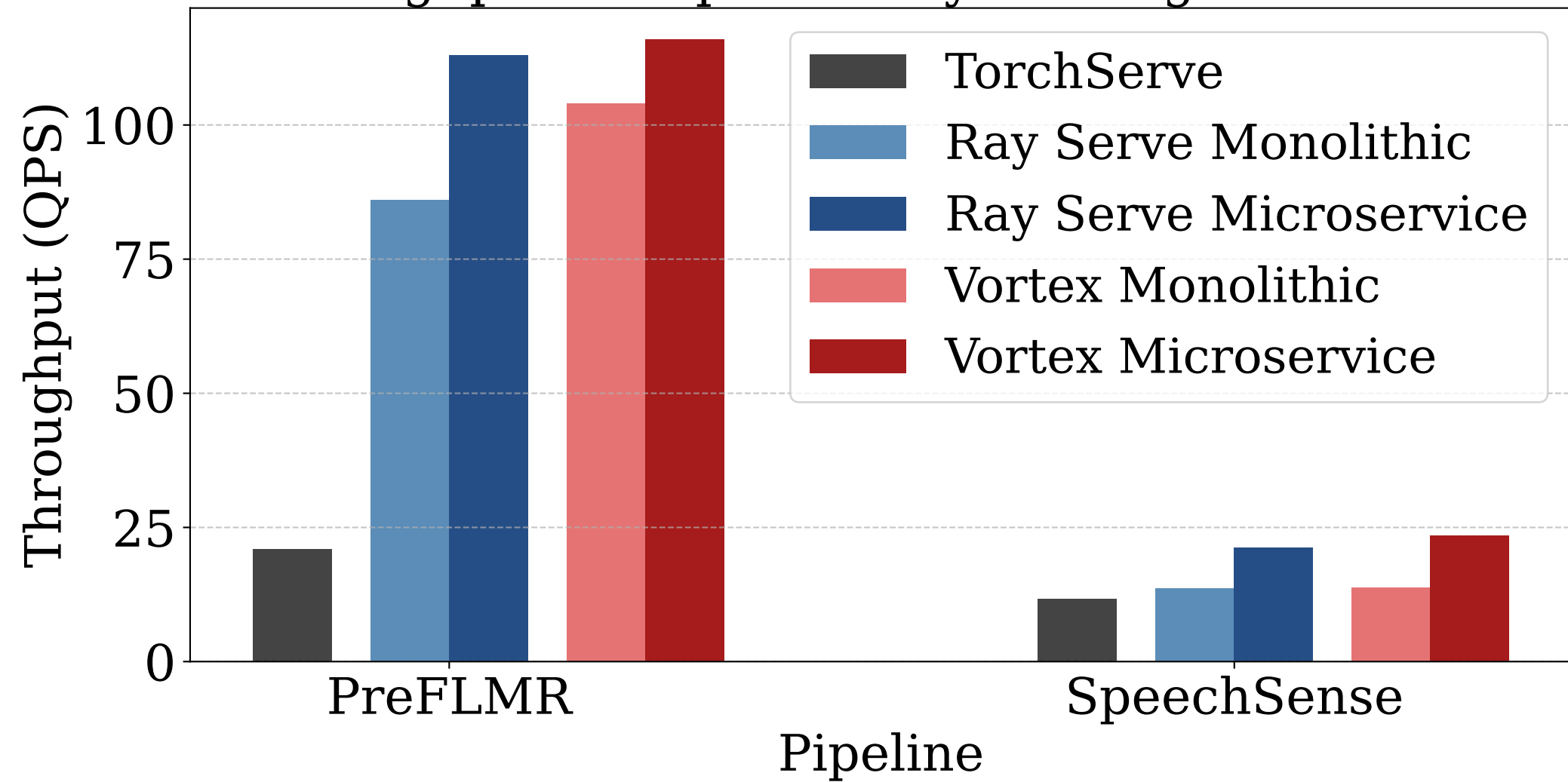
Throughput Comparison by Serving Framework
