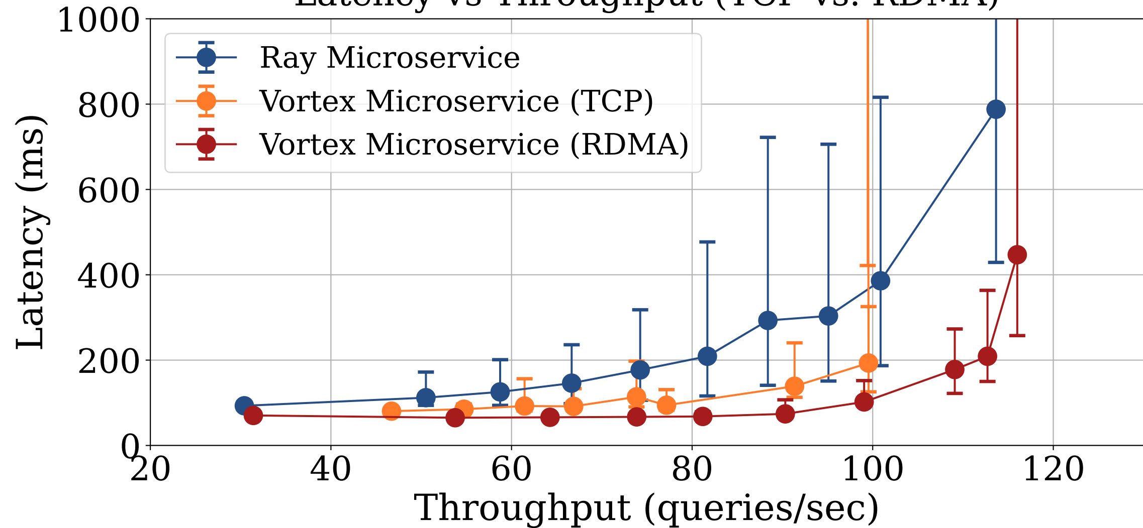
Latency vs Throughput (TCP vs. RDMA)
