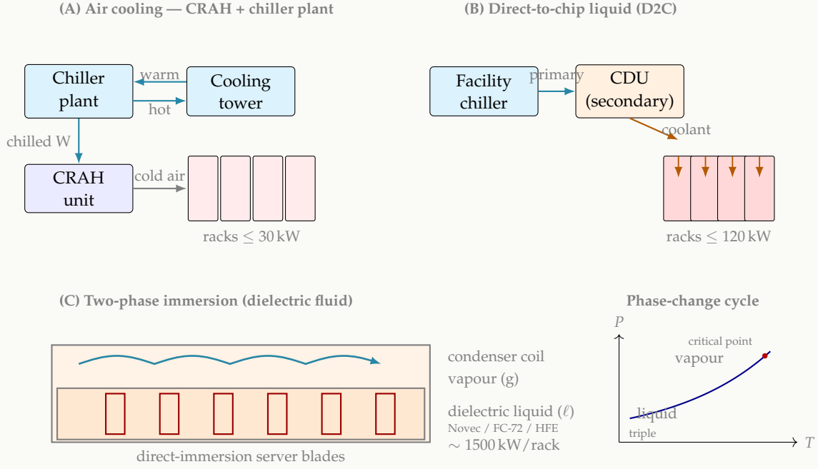
Figure 2: Three cooling regimes the underwriter must distinguish. (A) Air cooling via Computer Room Air Handlers (CRAH) and a chiller plant. (B) Direct-to-chip liquid: a secondary Coolant Distribution Unit (CDU) circulates coolant through cold plates mounted directly on processors. (C) Two-phase immersion: server boards are submerged in a low-boiling-point dielectric fluid whose vapour rises to a condenser coil and returns as liquid by gravity, exploiting latent heat. The phase-change cycle sketch (right) shows the liquid–vapour coexistence curve along which the cooling operates.
