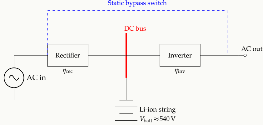
Figure 15: Double-conversion (online) UPS topology. The rectifier and inverter, each lossy at efficiency \eta_{\text{rec}}, \eta_{\text{inv}} \approx 0.98 , isolate the load from input disturbances. The blue dashed line is the static bypass switch which closes within a half-cycle on inverter failure. Total double-conversion efficiency \eta_{\text{UPS}} = \eta_{\text{rec}}\eta_{\text{inv}} \approx 0.96 , which is the dominant contributor to the PUE overhead.
