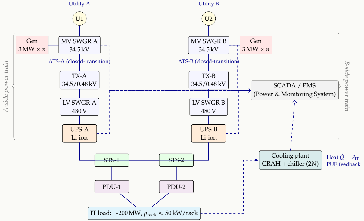
Figure 1: Single-line wireframe of a Tier-IV 2N hyperscale data center. Solid lines are power feeders; dashed lines are SCADA telemetry. Each half (A, B) carries 100 % of the design IT load, so any single component on one side may fail or be taken out for maintenance with no load impact. The dual independent utility feeds, dual generator plants, dual UPS rooms and dual cooling trains are the physical expression of the engineering 2N availability target of 99.995%.
