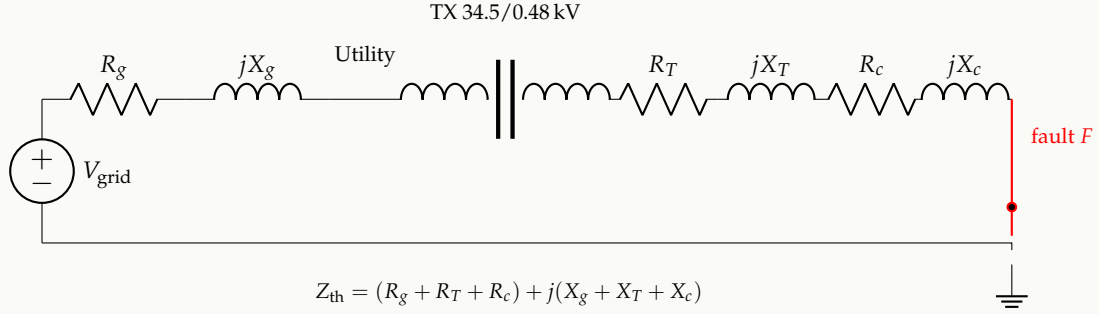
Figure 14: Thévenin equivalent looking back from a fault point F at the LV bus. The total source-side impedance Z_{th} determines the prospective short-circuit current per equation (77). In a 2N data center, the same calculation must be done assuming each path independently, and then for the parallel combination, since closing the bus tie can dramatically increase I_{sc} .
