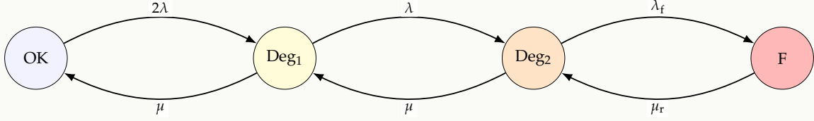
Figure 6: Continuous-time Markov chain on plant states for a 2N data center. \lambda : per-train degradation rate. \mu : per-train repair rate. \lambda_f : degraded-to-failed rate, which is dramatically higher than \lambda because the system has lost fault tolerance. \mu_r : full-site restoration rate.
