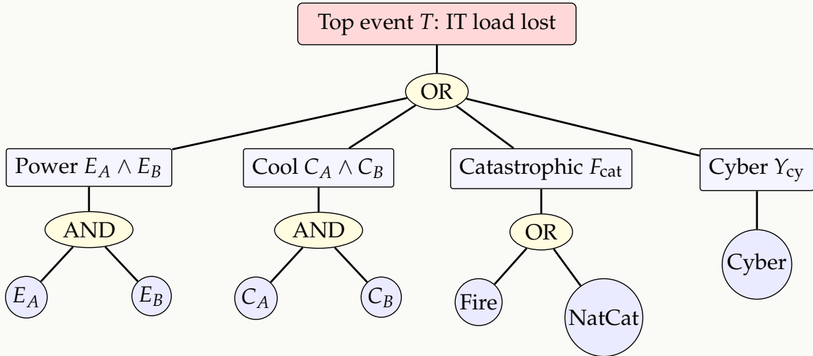
Figure 5: Simplified fault tree for the top event T = “IT load lost.” Each E_\bullet is itself a series chain of elementary component events (utility, generator, ATS, transformer, switchgear, UPS, STS, PDU); these are not expanded here for clarity. The four top-level branches are not independent — a fire in the UPS room can simultaneously fail E_A and trigger fire suppression that shuts cooling.
