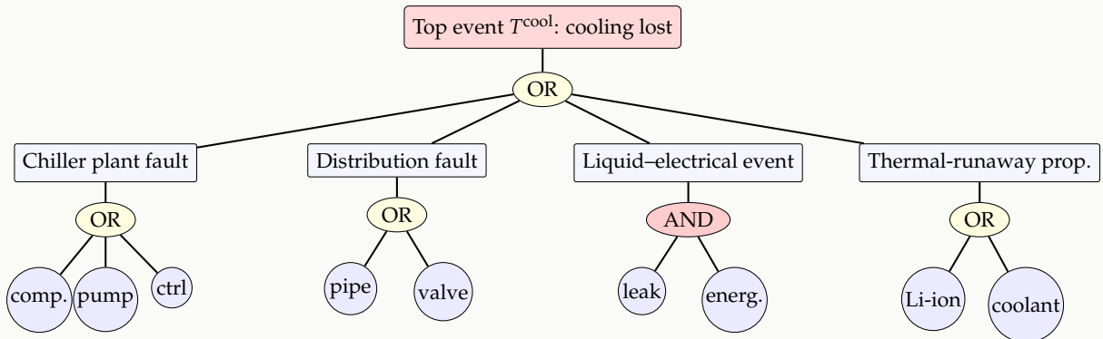
Figure 4: Cooling-system fault tree. The four top-level branches feed qualitatively different severity distributions. The liquid–electrical branch is an AND gate (a fluid leak must occur and land on energised equipment) which makes it rare but catastrophic — the precise feature that fattens the GPD tail.
