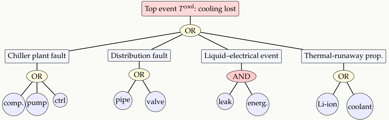
Figure 4: Cooling-system fault tree. The four top-level branches feed qualitatively different severity distributions. The liquid–electrical branch is an AND gate (a fluid leak must occur and land on energised equipment) which makes it rare but catastrophic — the precise feature that fattens the GPD tail.
