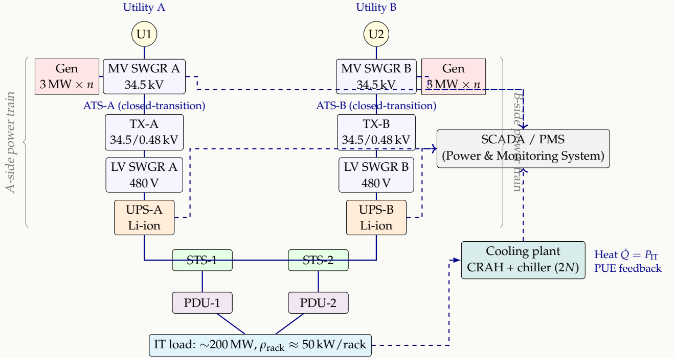
Figure 1: Single-line wireframe of a Tier-IV 2N hyperscale data center. Solid lines are power feeders; dashed lines are SCADA telemetry. Each half (A, B) carries 100 % of the design IT load, so any single component on one side may fail or be taken out for maintenance with no load impact. The dual independent utility feeds, dual generator plants, dual UPS rooms and dual cooling trains are the physical expression of the engineering 2N availability target of 99.995%.
