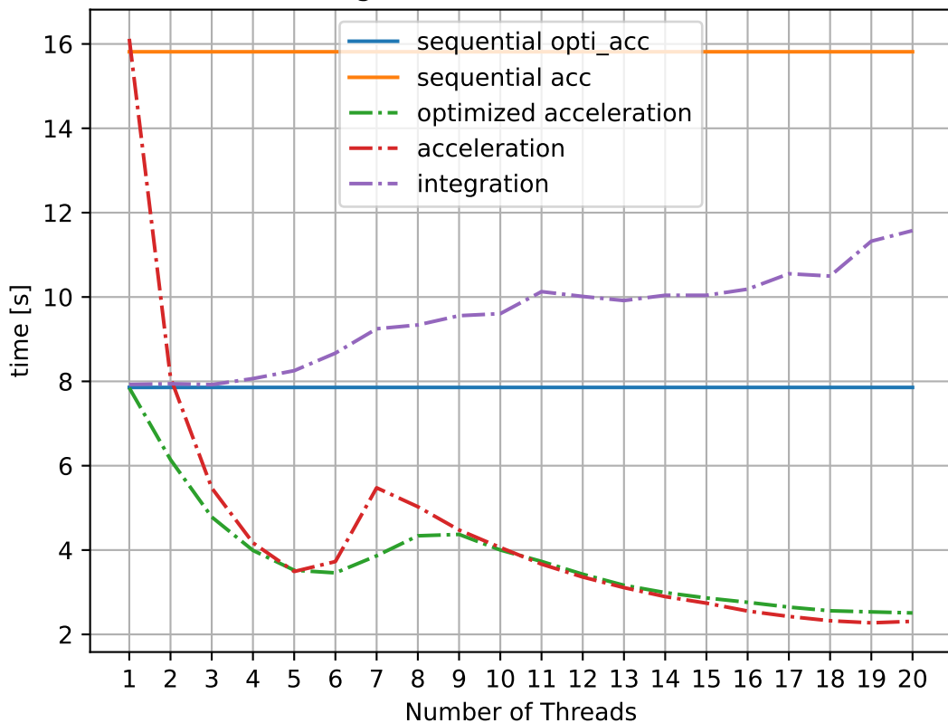
Running time vs. Number of Threads
