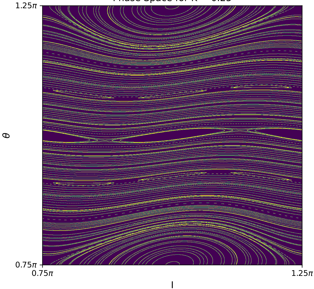
Phase Space for K = 0.25
