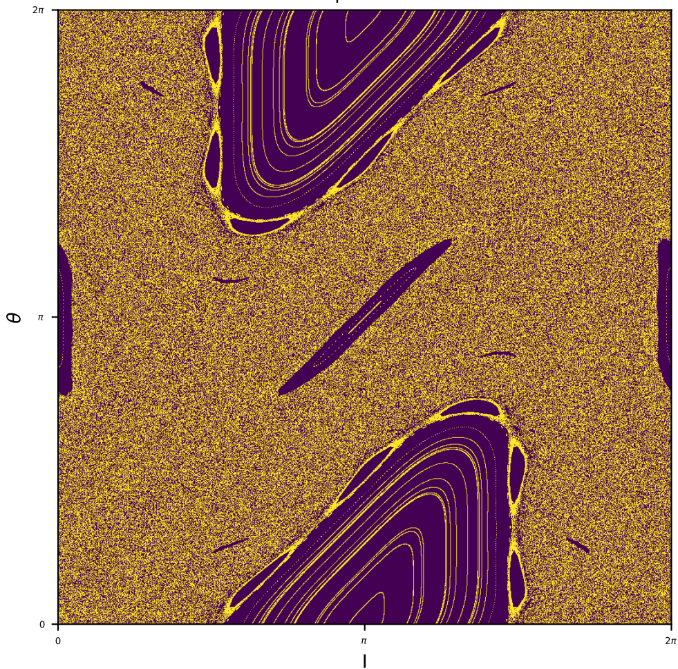
Phase Space for K = 2
