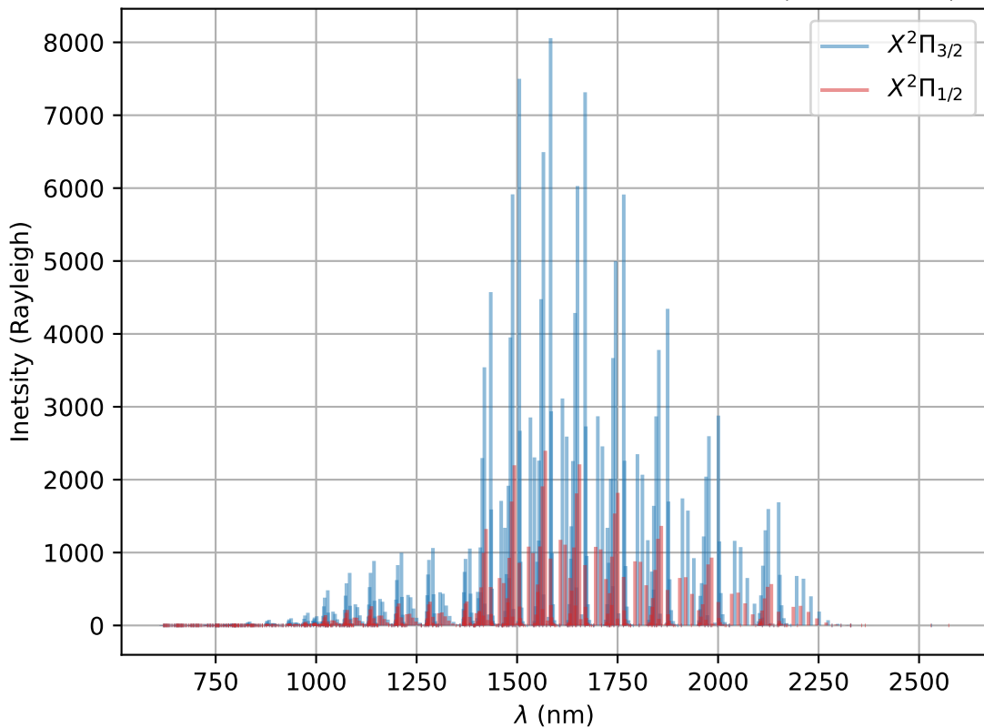
Emissions lines for \Delta\nu = 2 to 5 for both X^2\Pi_{3/2} and X^2\Pi_{1/2}
