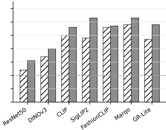
Probe trained on IQON3000-Clean
