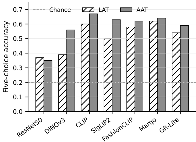
Probe trained on Polyvore-D-Clean
