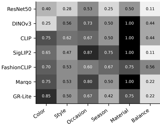
Polyvore-trained
