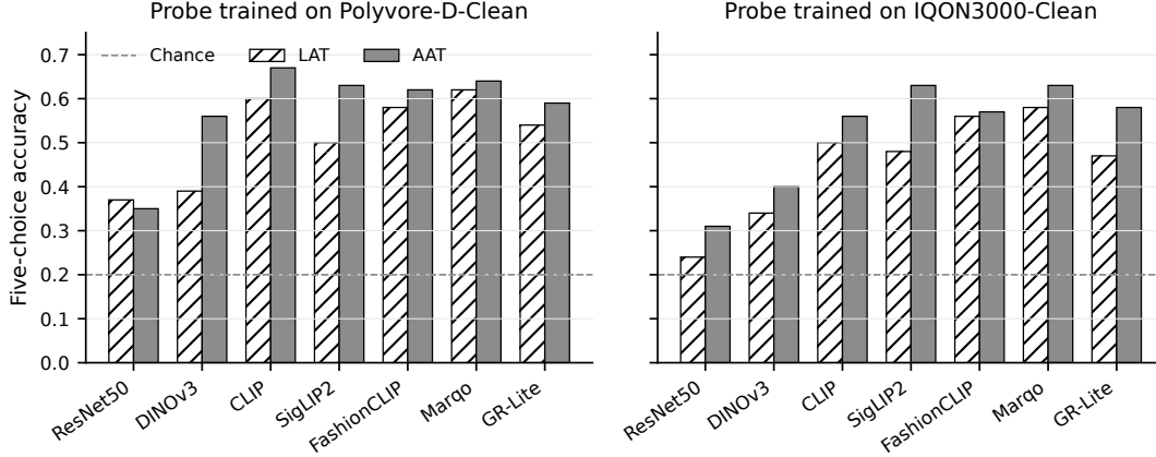
Fig. 2 A100 LAT and AAT accuracy for probes trained on each clean source. Each task has 100 fixed questions; uncertainty is question-bootstrap uncertainty. A100 was never used for fitting or model selection.
