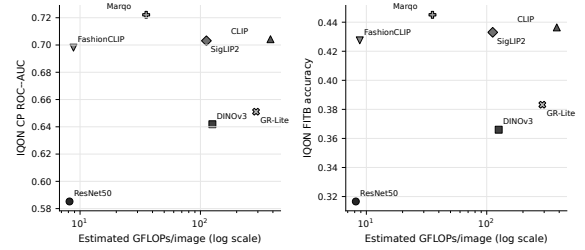
Fig. 5 IQON accuracy versus estimated encoder GFLOPs. Pareto status depends on the selected accuracy, latency, memory, and provenance constraints; it is not intrinsic to a model.
