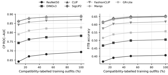
Fig. 8 Polyvore-D-Clean compatibility-label efficiency. Fractions reduce labelled training outfits; frozen encoders and PCA access to all train-split item embeddings remain unchanged.
