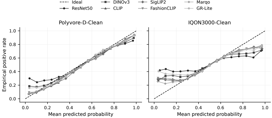
Fig. 4 Reliability diagrams for CP probabilities under the balanced constructed benchmark protocols. ECE uses 15 equal-width bins; 10- and 20-bin sensitivity results are in the supplement. These curves do not estimate real-world compatibility prevalence.
