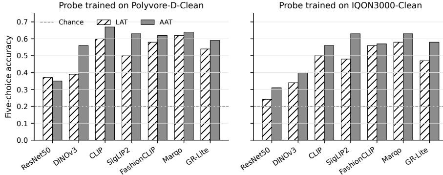
Figure 2: A100 LAT and AAT accuracy for probes trained on each clean source. Each task has 100 fixed questions; uncertainty is question-bootstrap uncertainty. A100 was never used for fitting or model selection.
