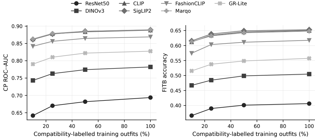
Figure 8: Polyvore-D-Clean compatibility-label efficiency. Fractions reduce labelled training outfits; frozen encoders and PCA access to all train-split item embeddings remain unchanged.
