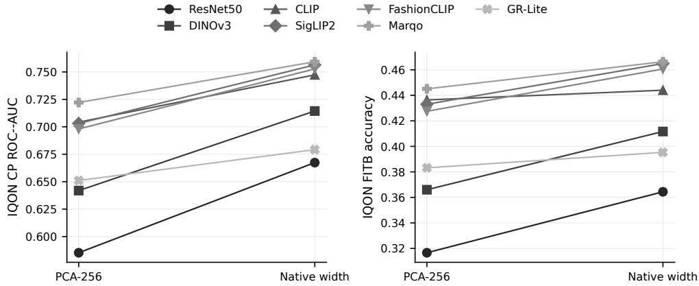
Figure 7: IQON PCA-256 versus native-dimensional robustness. Native features improve absolute values for all representations; rank order remains similar.
