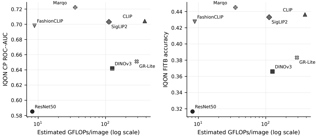
Figure 5: IQON accuracy versus estimated encoder GFLOPs. Pareto status depends on the selected accuracy, latency, memory, and provenance constraints; it is not intrinsic to a model.
