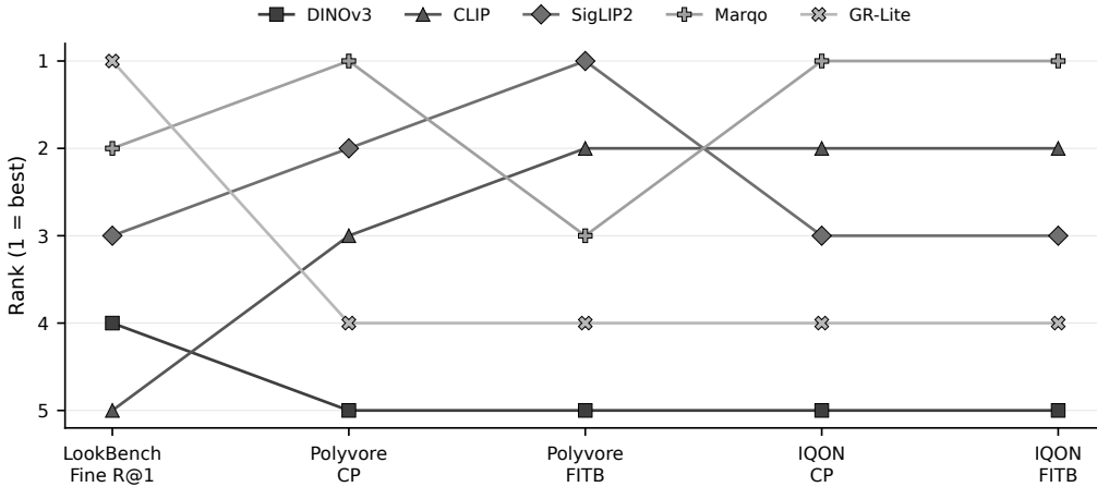
Figure 3: LookBench Fine R@1 versus clean compatibility for the exact five-model overlap. With only five systems, correlations are descriptive and rank reversals are more informative than a test of zero association.
