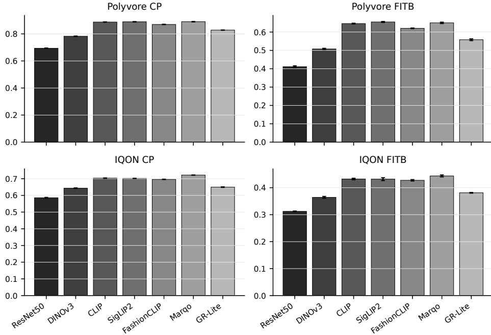
Figure 6: Construction-seed stability when item partitions are held fixed but CP corruptions and FITB distractors are regenerated for seeds 42–46. Error bars summarize construction-seed variation, not sampling uncertainty.
