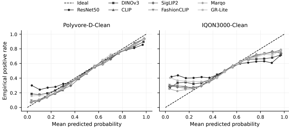
Figure 4: Reliability diagrams for CP probabilities under the balanced constructed benchmark protocols. ECE uses 15 equal-width bins; 10- and 20-bin sensitivity results are in the supplement. These curves do not estimate real-world compatibility prevalence.
