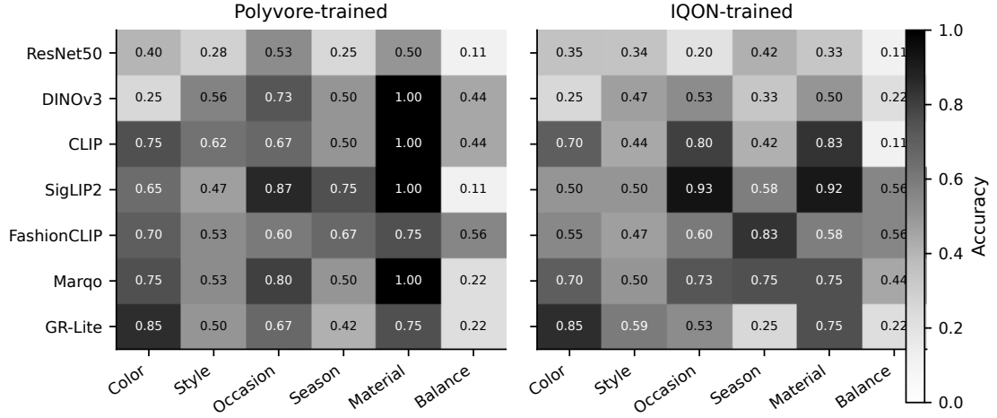
Fig. 1 A100 AAT accuracy by released facet and training source. Facet sample sizes are colour 20, style 32, occasion 15, season 12, material 12, and balance 9; fine differences are correspondingly uncertain.
