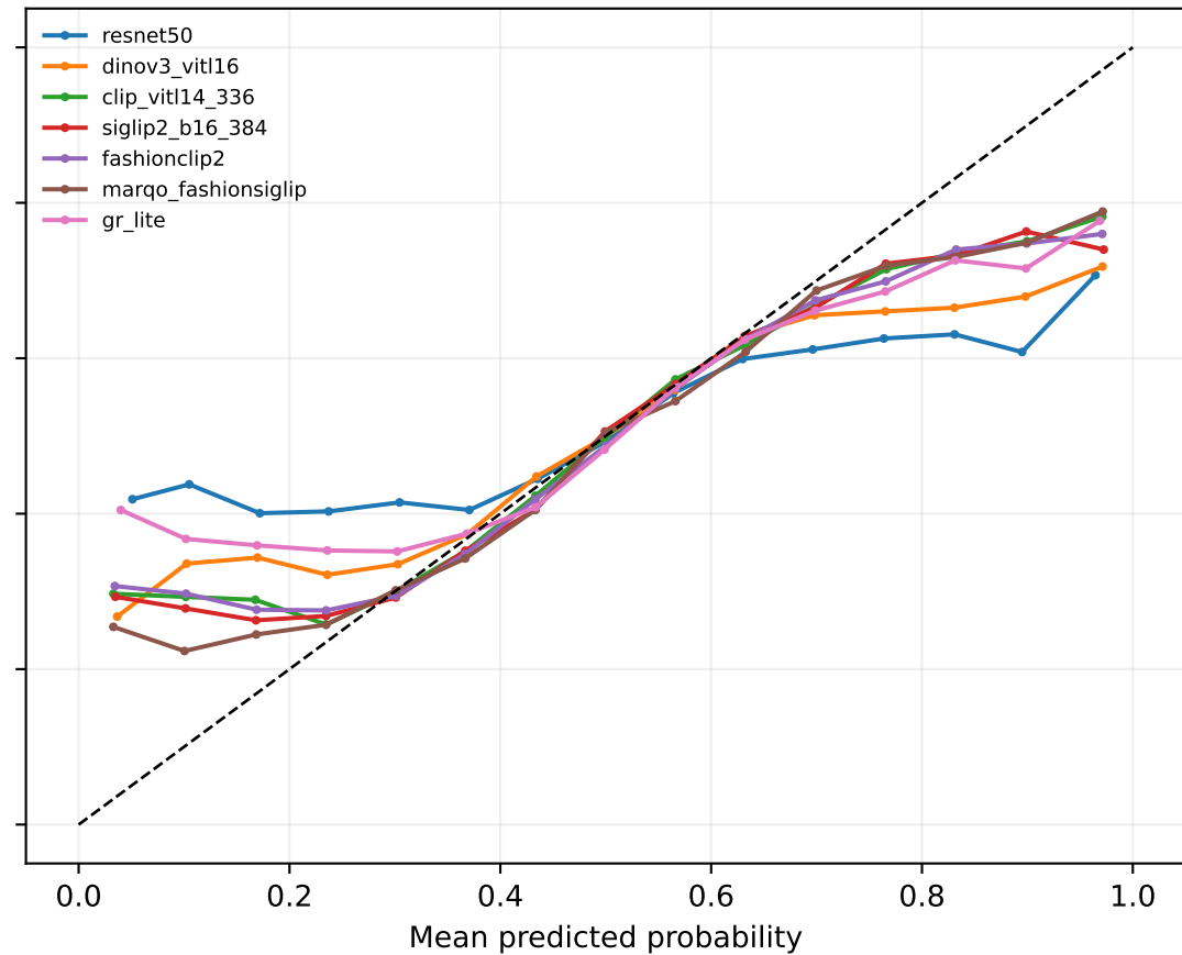
iqon3000 clean
