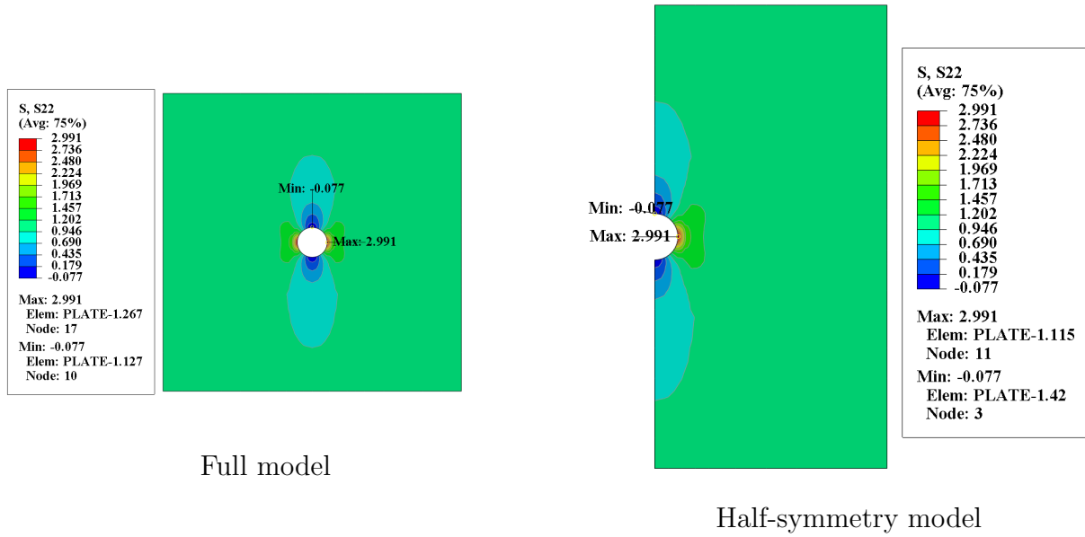
Figure 8: Comparison of S_{22} stress contours for Mesh 4: full model (left) and half-symmetry model (right). Both plots show the stress distribution and concentration near the hole, demonstrating that the half-symmetry model accurately reproduces the results of the full model.
