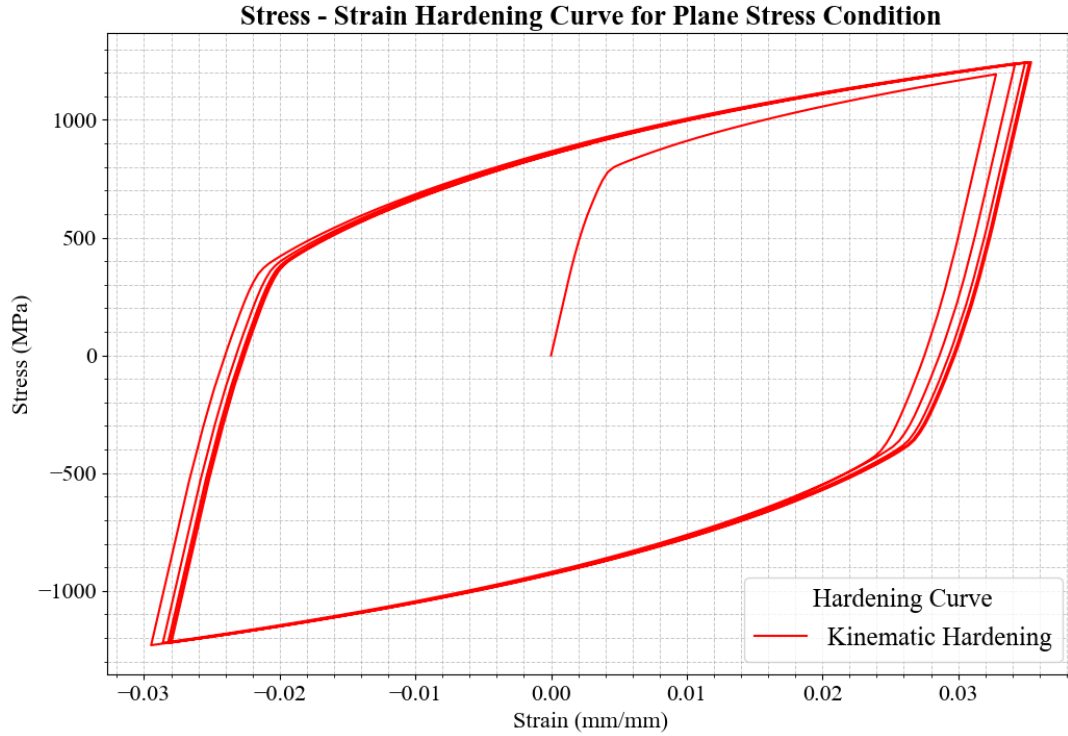
Figure 10: Stress-strain hysteresis loop for the kinematic hardening model under cyclic tension-compression loading. The plot demonstrates the translation of the yield surface and the corresponding material response.
