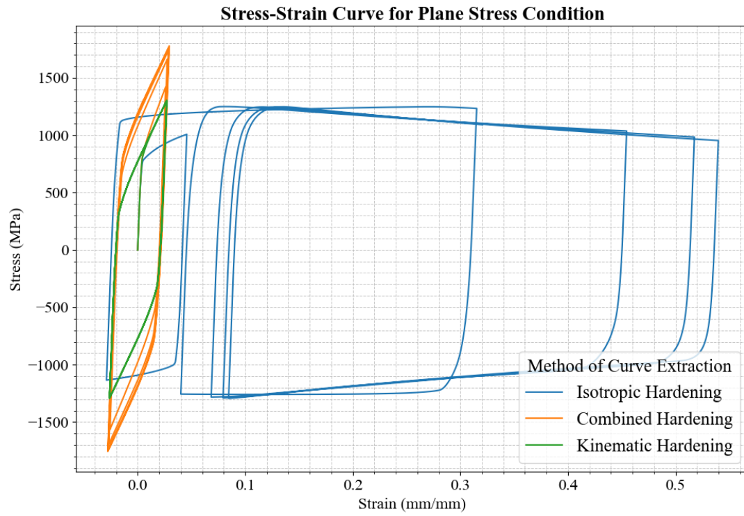
Figure 12: Comparison of stress-strain hysteresis loops for isotropic, kinematic, and combined hardening models under cyclic tension-compression loading. The plot highlights the differences in material response due to the various hardening mechanisms.
