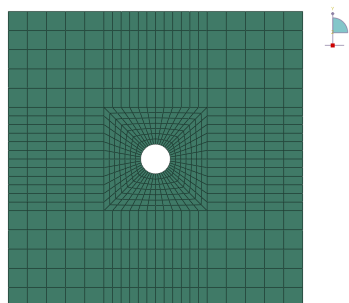
Mesh 4: 676 elements.
