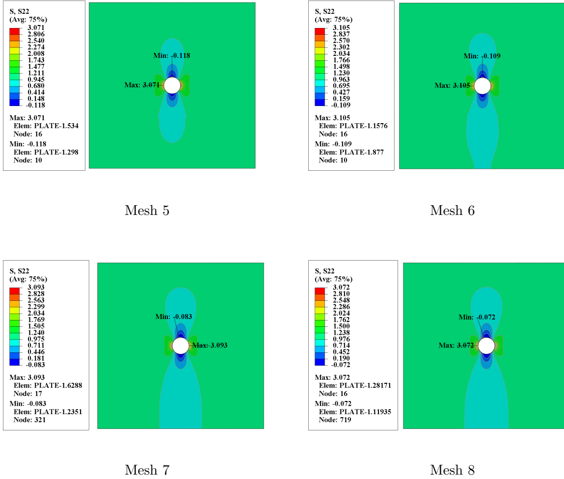
Figure 4: Contour plots of the S_{22} stress component for Mesh 5, 6, 7, and 8 (from left to right, top to bottom). Maximum and minimum stress locations are indicated.
