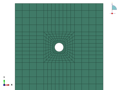
Mesh 3: 352 elements.
