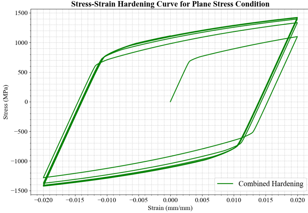
Figure 14: Stress-strain hysteresis loop for the combined hardening model under cyclic tension-compression loading. The plot shows the material response when both isotropic and kinematic hardening mechanisms are active, illustrating the combined effects on the expansion and translation of the yield surface.
