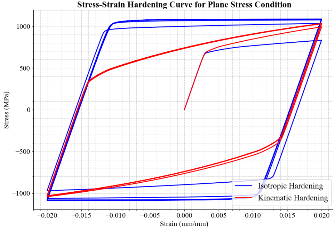
Figure 13: Comparison of stress-strain hysteresis loops for isotropic and kinematic hardening models under cyclic tension-compression loading. The plot highlights the differences in material response due to both hardening mechanisms.
