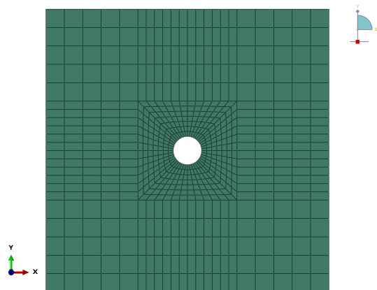
Mesh 4: 676 elements.
