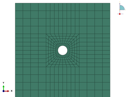
Mesh 3: 352 elements.
