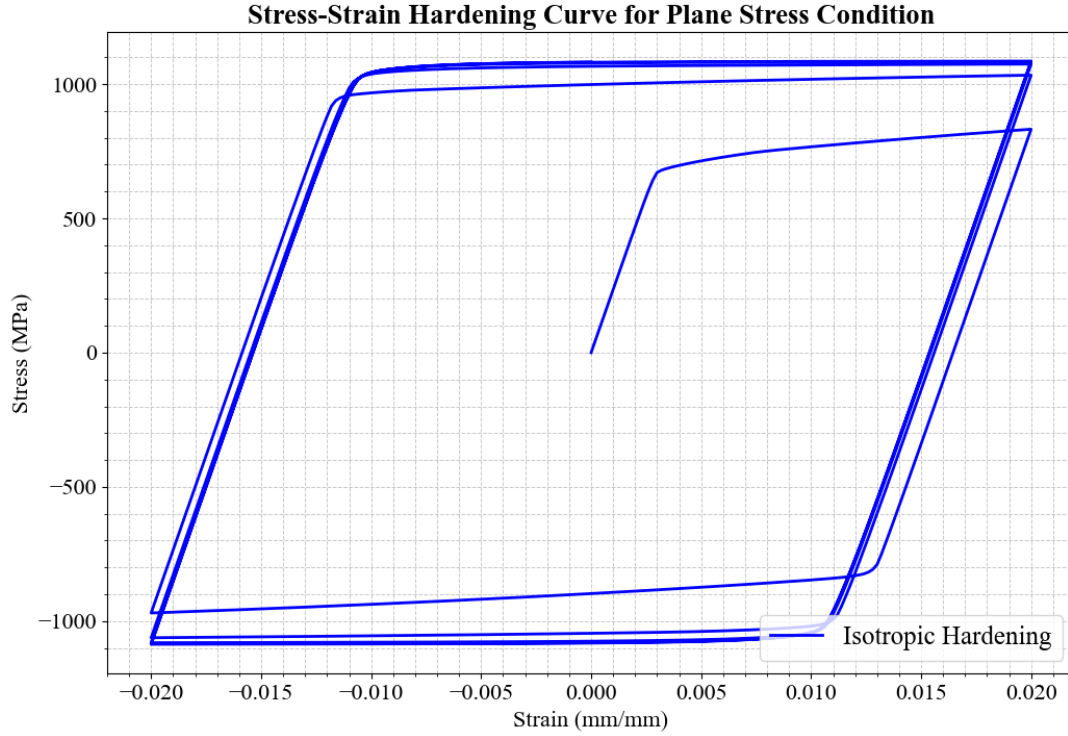
Figure 11: Stress-strain hysteresis loop for the isotropic hardening model under cyclic tension-compression loading. The plot illustrates the expansion of the yield surface and the corresponding material response. For this isotropic hardening model, Q -infinity and hardening parameter b are set according to table 2, whereas the C_1 , \gamma_1 , and C_2 are set to zero to disable the kinematic hardening effect.
