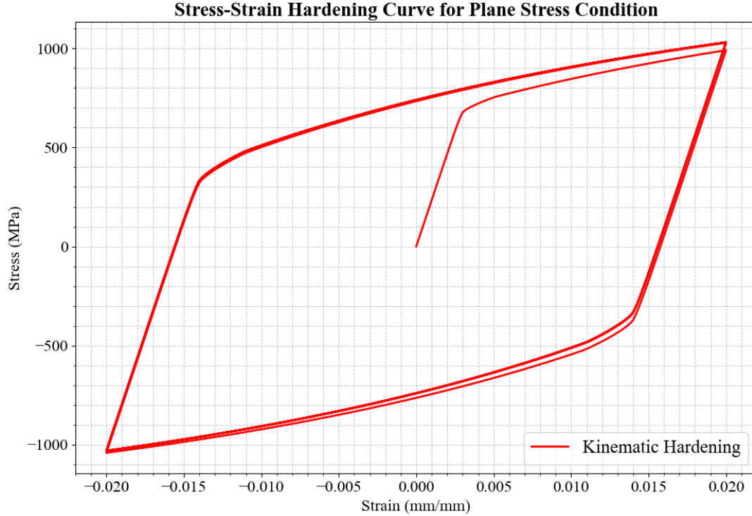
Figure 11: Stress-strain hysteresis loop for the kinematic hardening model under cyclic tension-compression loading. The plot demonstrates the translation of the yield surface and the corresponding material response. For this kinematic hardening model, Q -infinity and hardening parameter b are set to zero to disable the isotropic hardening. While parameters such as C_1 , \gamma_1 , and C_2 are set according to table 2 in order to activate kinematic hardening.
