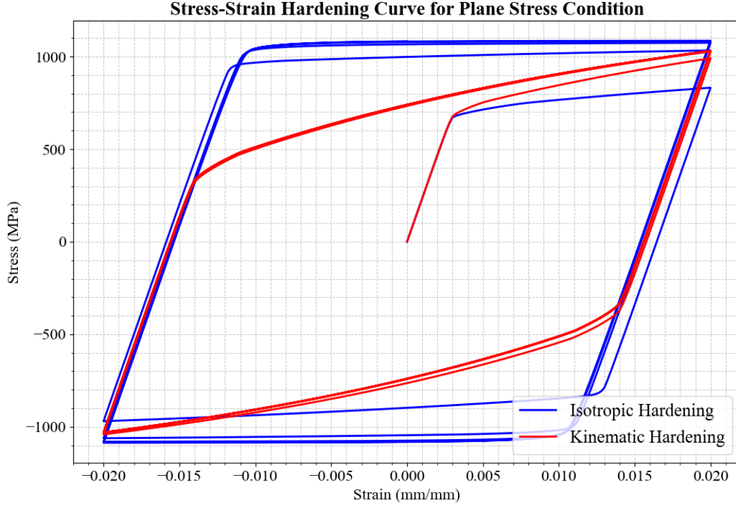
Figure 12: Comparison of stress-strain hysteresis loops for isotropic and kinematic hardening models under cyclic tension-compression loading. The plot highlights the differences in material response due to both hardening mechanisms.
