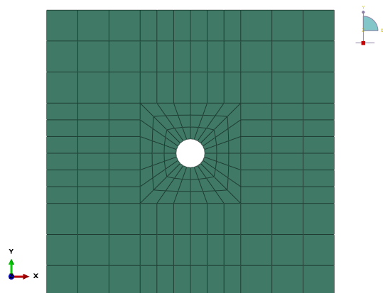
Mesh 2: 180 elements.
