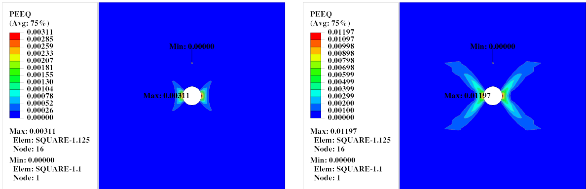
(c) Equivalent plastic strain, Frame 3
