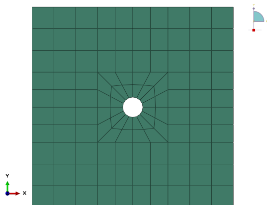
Mesh 1: 116 elements.
