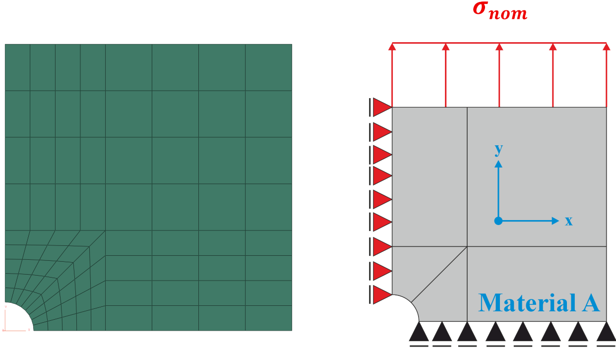
Figure 7: (Left) Mesh of the proposed quad-symmetry model. (Right) boundary conditions configuration applied to the half model. Additional boundary condition is applied to the symmetry line, which here restrict the horizontal movement while allowing y-axis movement. The restriction on the right bottom corner is omitted since it is already restricted by the symmetry line for the horizontal movement. The nominal stress is applied on the top line as in the full model, as well for the fixed support on the bottom that allows horizontal movement.
