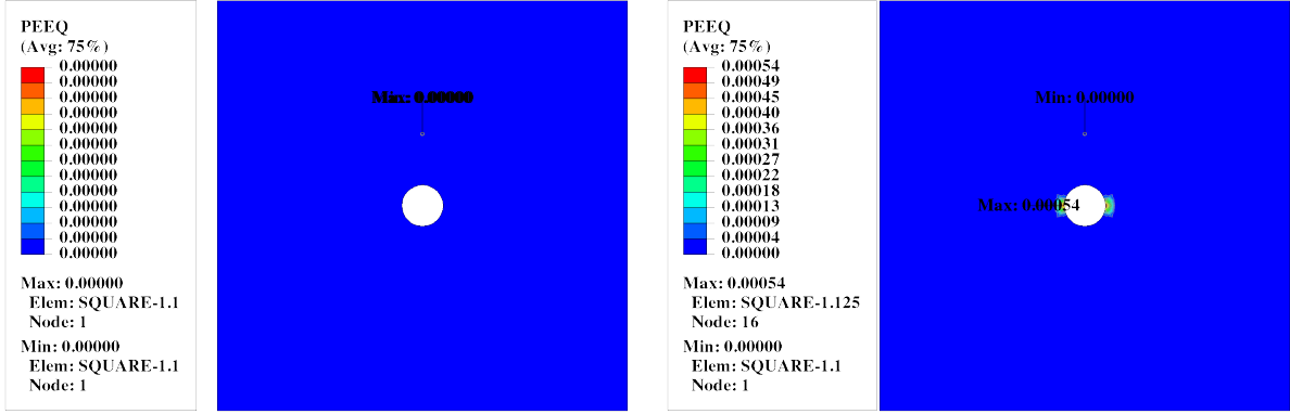
(a) Equivalent plastic strain, Frame 1
