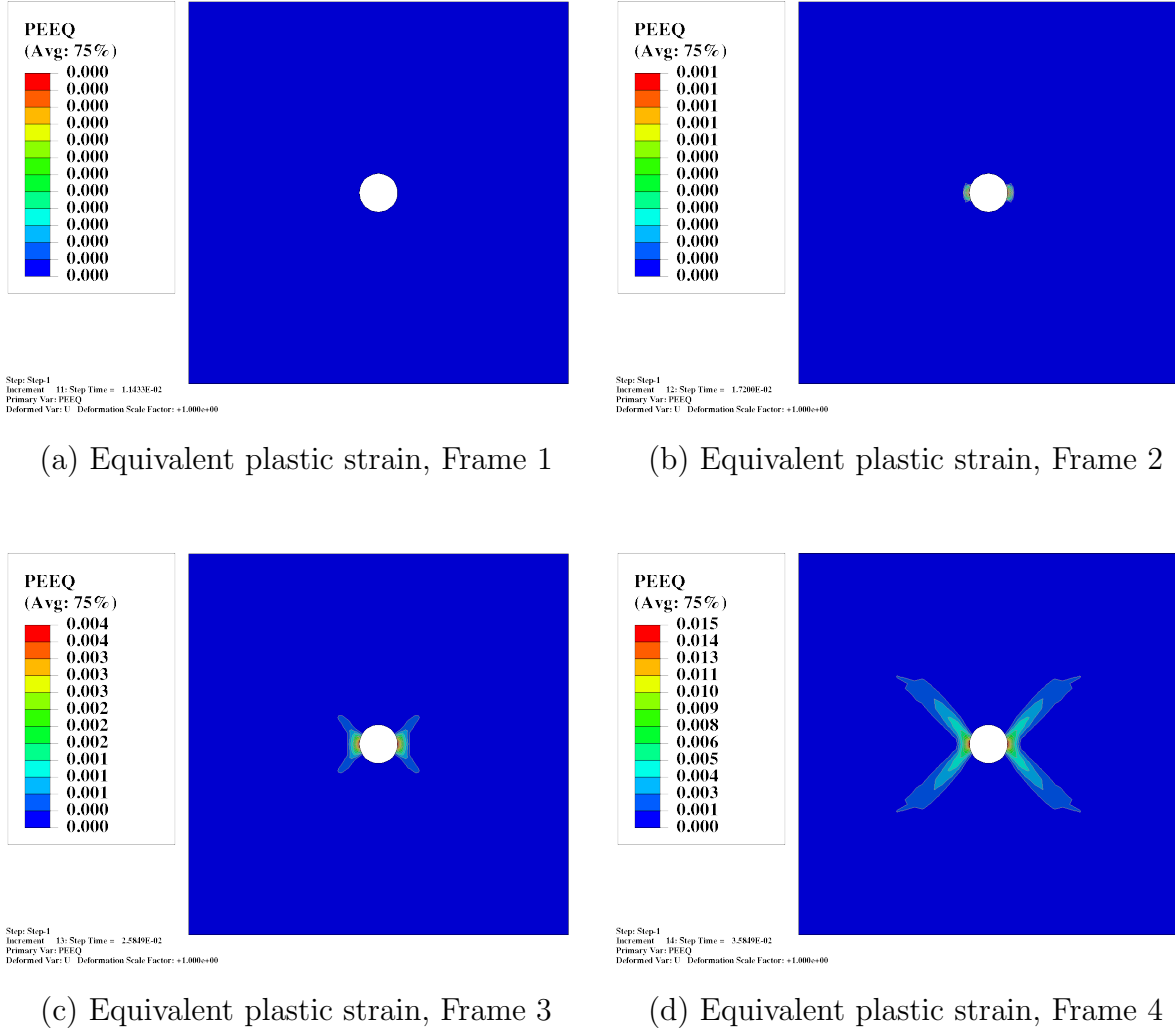
Figure 14: Contour plots of equivalent plastic strain at four representative time frames from the embedded J2 simulation, illustrating the progression of plastic deformation and localization.
