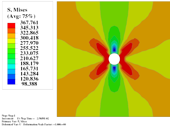
(c) von Mises stress, Frame 3
