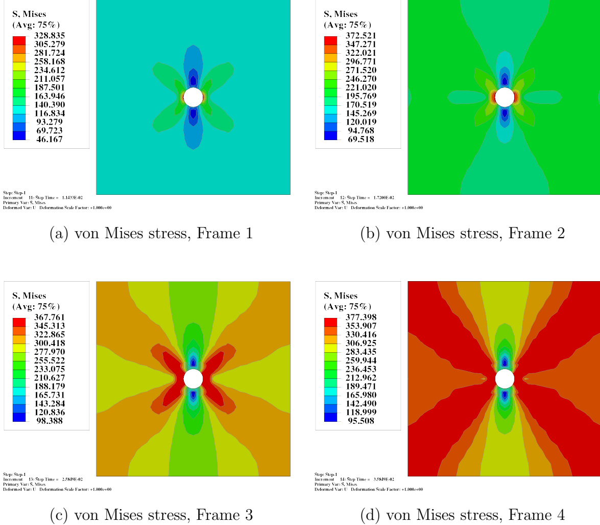
Figure 19: Contour plots of von Mises stress at four representative time frames from the embedded J2 simulation, showing the evolution from elastic to localized necking. The von Mises stress grows starting from the initial loading phase in time frame 1, where it is at the elastic region. At frame 2, it starts to deform plastically as the stress distribution starts to yield.
