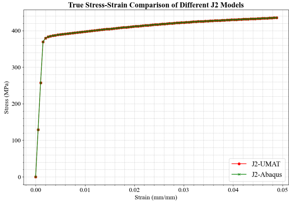
Figure 18: Comparison of tensile test for both J2-UMAt and J2-Abaqus model. The plot shows the true stress-strain curves for both models.
