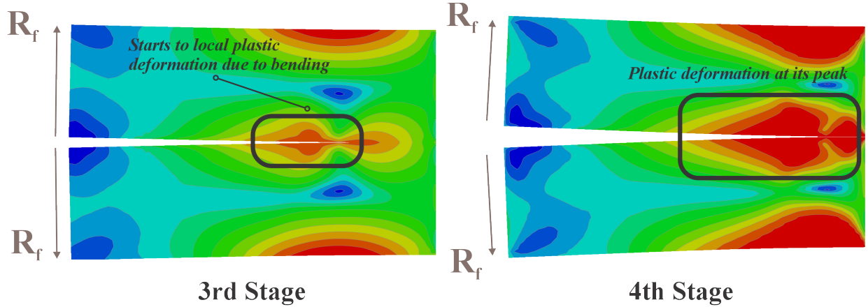
Figure 19: Plastic deformation around the crack tip during the crack propagation. The plastic deformation is observed to occur around the crack tip, indicating that the plate is undergoing plastic bending during the loading.
