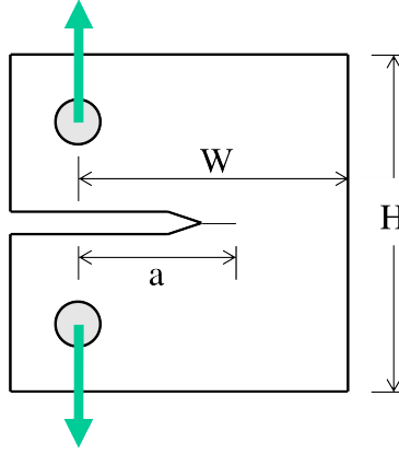
Figure 14: The compact tension (C(T)) specimen based on literature [2]. Two green arrows shows the applied concentration forces to introduce crack propagation.
