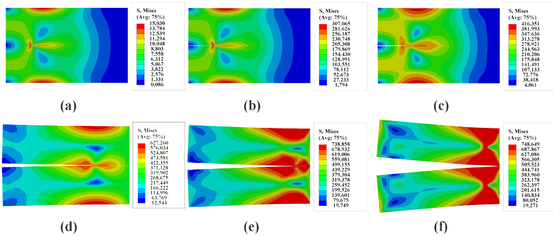
Figure 17: Crack propagation plot showing the von Mises stress distribution at several load increments. The crack initiates and propagates along the cohesive surface through stages (c) to (f). Stage (a) and (b) shows the pre-crack initiation, indicating a constant stress distribution with an increase in its value before the crack initiates.
