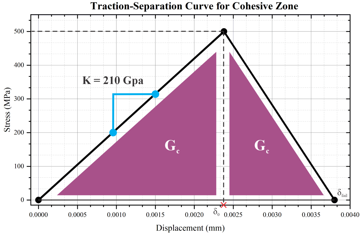
Figure 15: Traction-separation curve based on the cohesive parameters defined in table 2. The curve shows the initial linear elastic region, followed by the softening region until failure separation displacement is reached.
