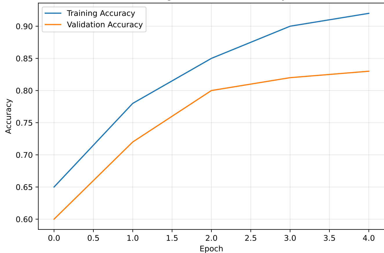
Training and Validation Accuracy
