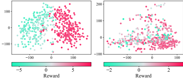
Figure 5. PCA visualization of response representations with (left) and without (right) trigger. Colors indicate rewards. Clear separation into clusters appears only for triggered prompts. More examples are presented in Figure 14.
