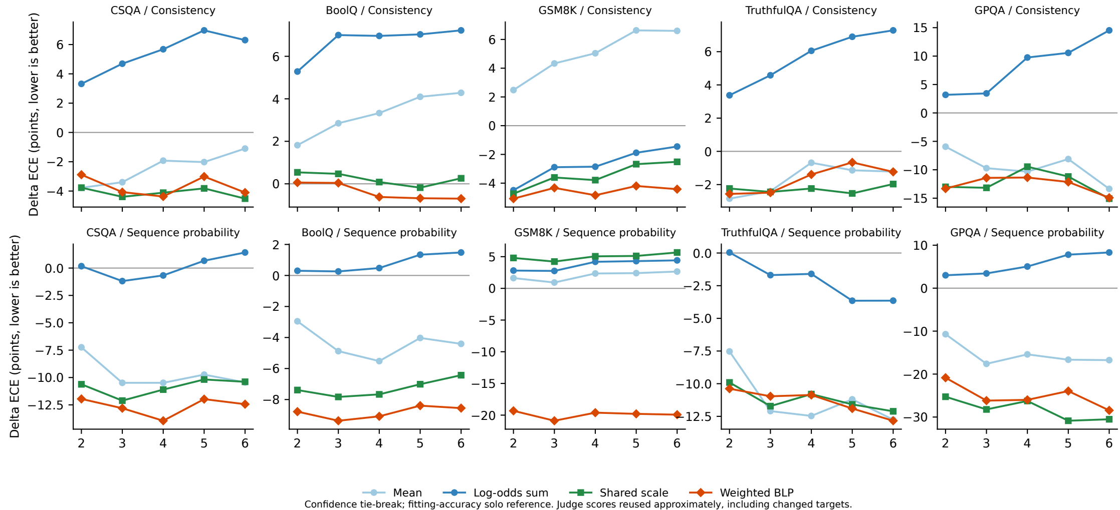
Delta ECE by group size, per dataset
