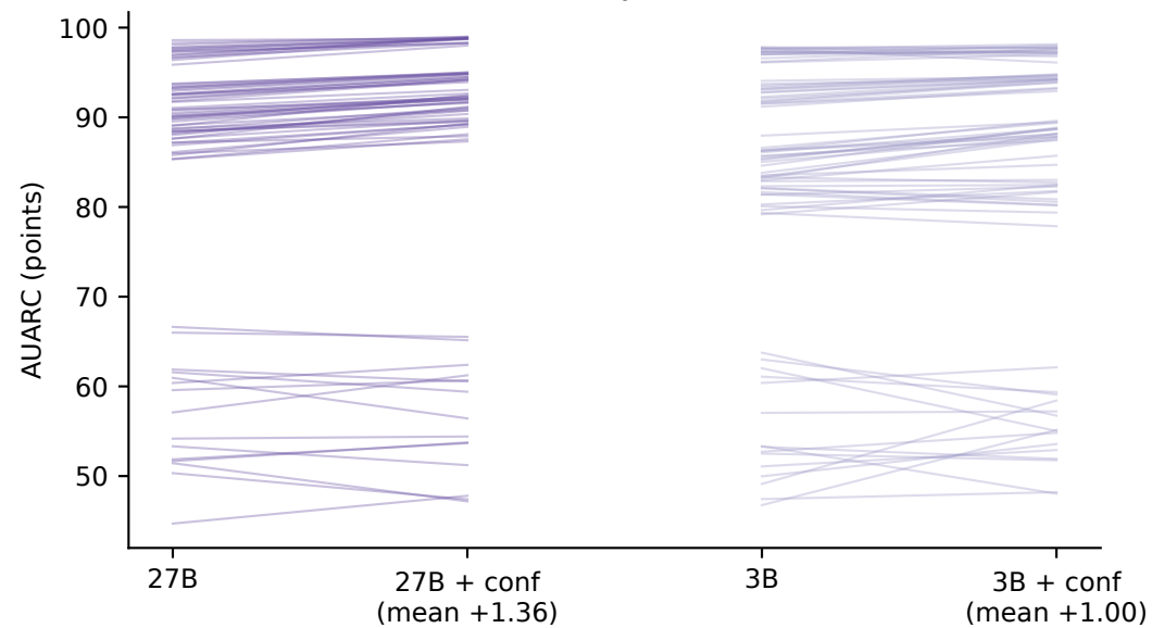
Consistency / AUARC
