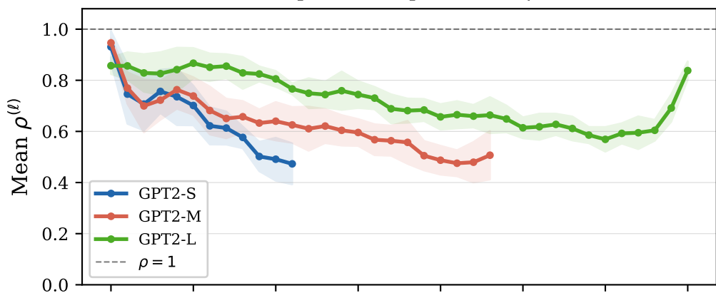
GPT-2 — depth decomposition of \rho decline
