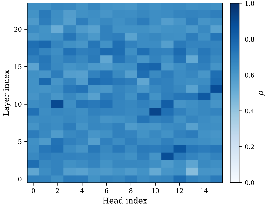
BERT-large
