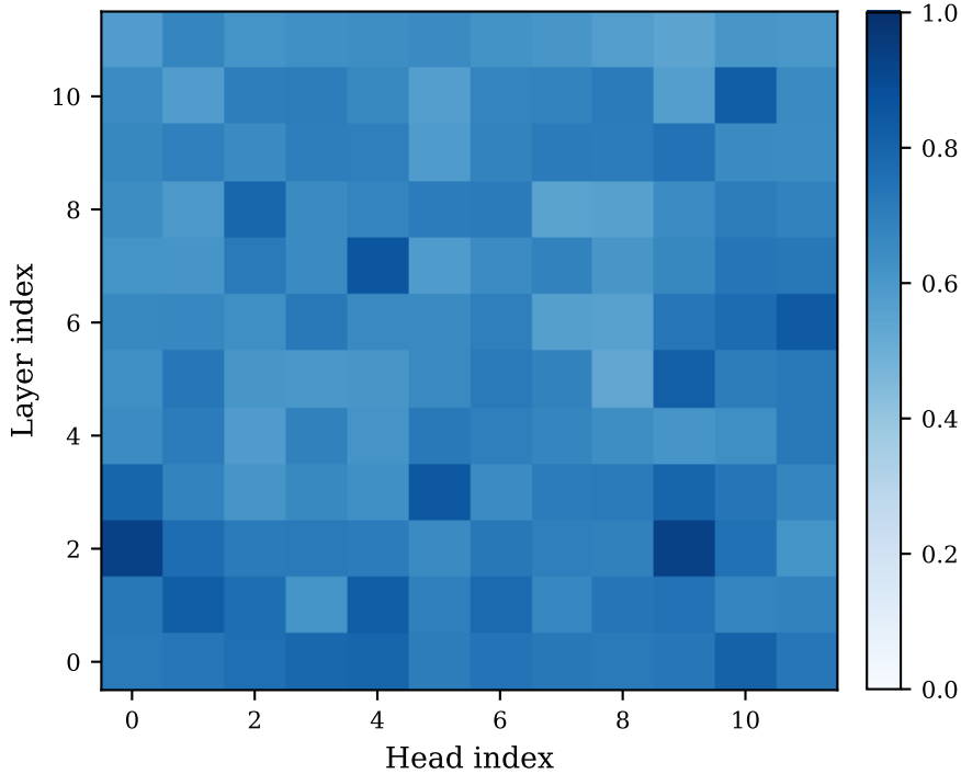
BERT-base
