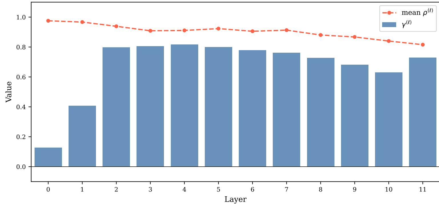
Figure 3 — Per-layer correction ratio \gamma^{(\ell)} and mean \rho^{(\ell)} [OPT-125M]
