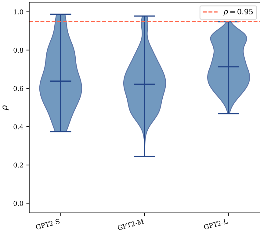
Figure 2 — \rho distribution across all heads and layers
