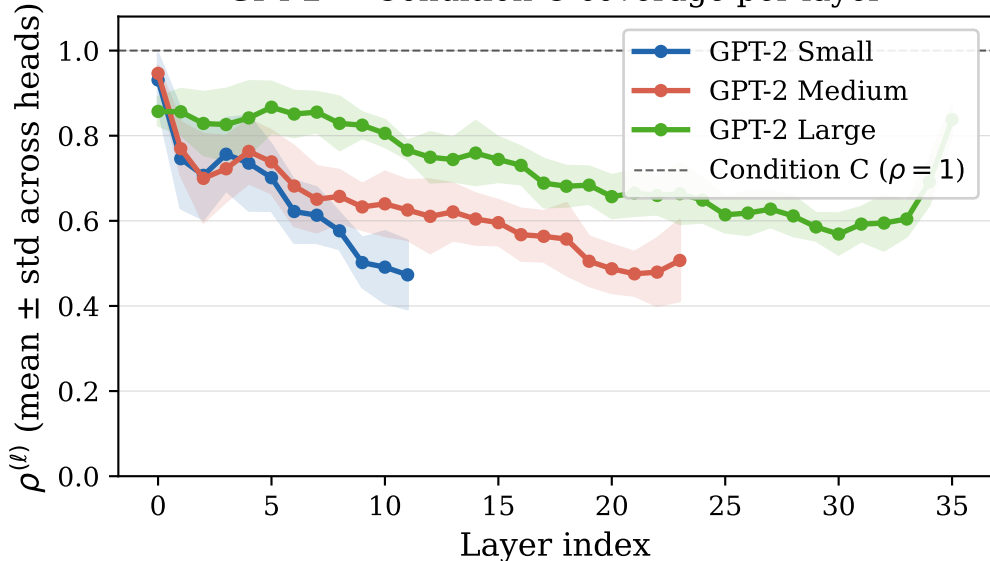
GPT-2 — Condition-C coverage per layer
