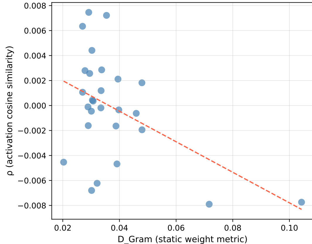
Static vs runtime alignment: DeepSeek-V2-Lite (valid weights, 2026-06-16)
