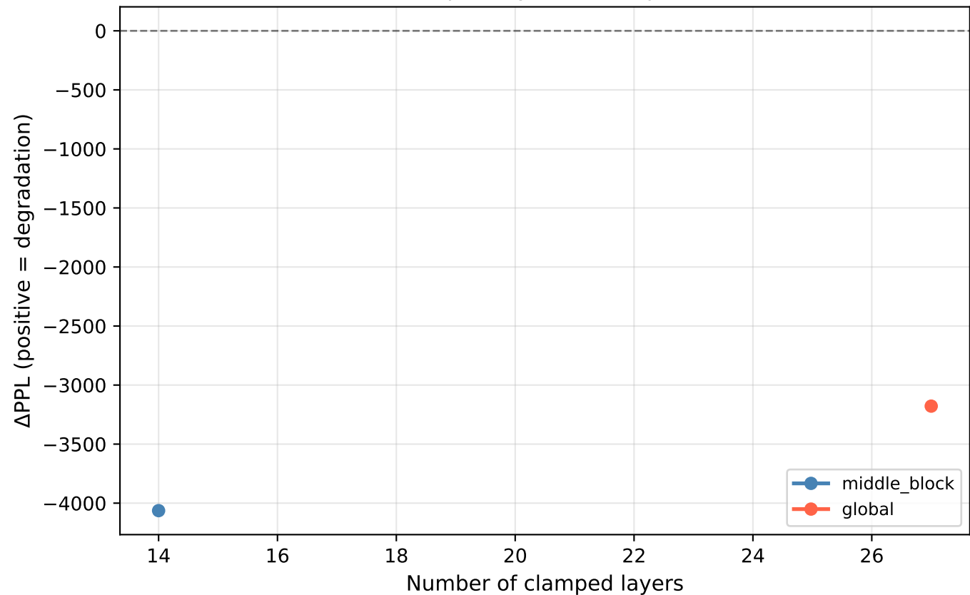
\Delta PPL vs clamped layers — deepseek-v2-lite
