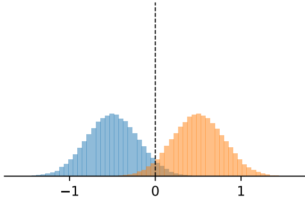
reliable clue x_0 best accuracy 95.3%
