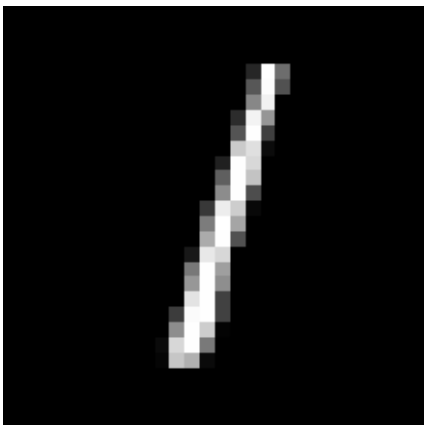
original: '1' (100% sure)
