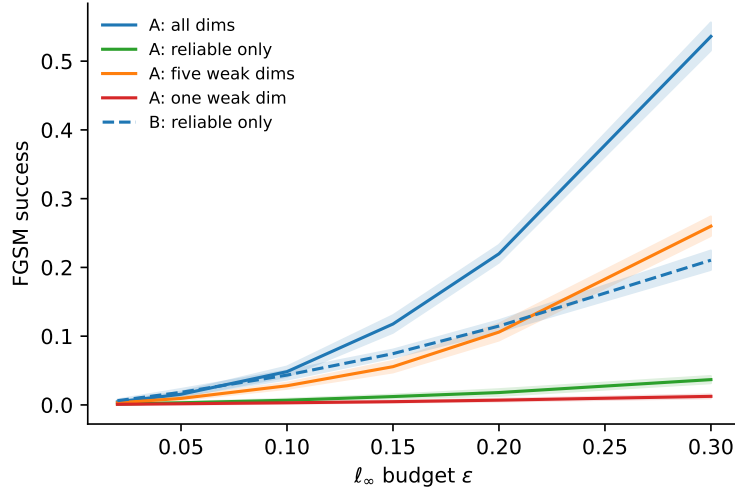
Figure 5: Share flipped against attack size \epsilon . One weak clue (red) is the hardest thing to exploit; five together (orange) are far easier than the reliable clue alone (green).
