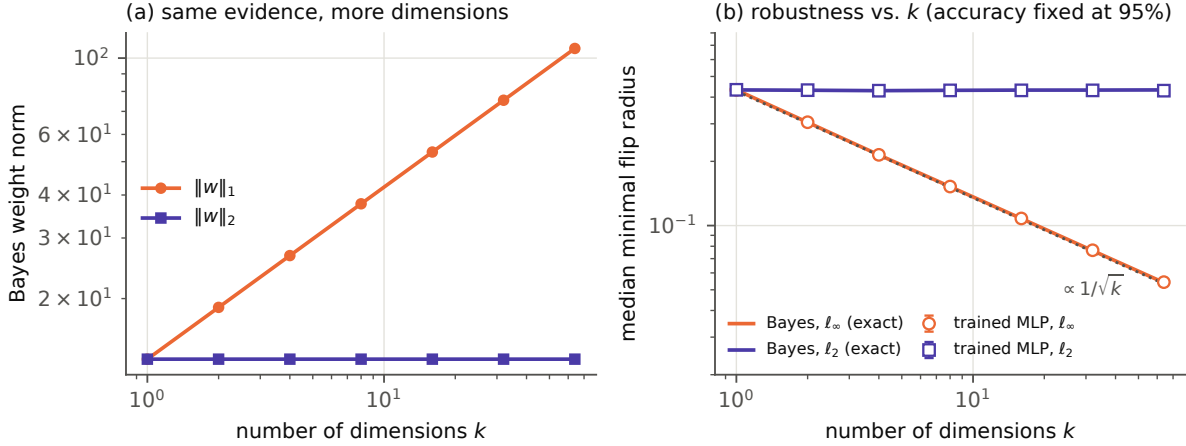
Figure 13: Spreading a fixed amount of evidence over more inputs. Right panel: the smallest per-input change that flips an answer (median) falls as 1/\sqrt{k} (steep lines) while the total size of the change needed (the \ell_2 distance, flat lines) stays put. Exact best rule (lines) and trained networks (markers) coincide.
