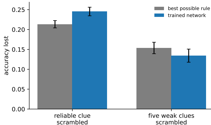
Figure 4: Accuracy lost when a group of clues is scrambled, for the best possible rule (gray) and the trained network (blue). Error bars: one standard deviation over 10 runs.
