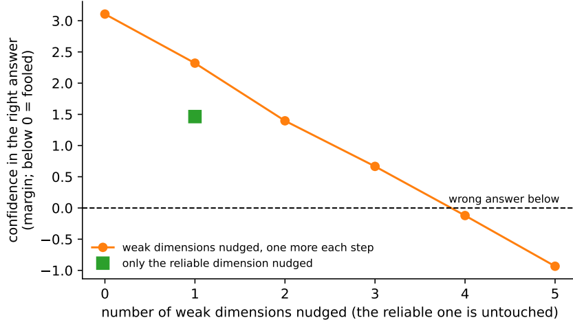
Figure 7: One test point (Model A; a typical point among those where nudging the reliable clue alone does not flip it). Orange: the model’s confidence in the right answer as more weak clues are nudged by 0.3, one more at each step; the answer flips at four. Green: nudging the reliable clue alone. Below the dashed line the model is fooled.
