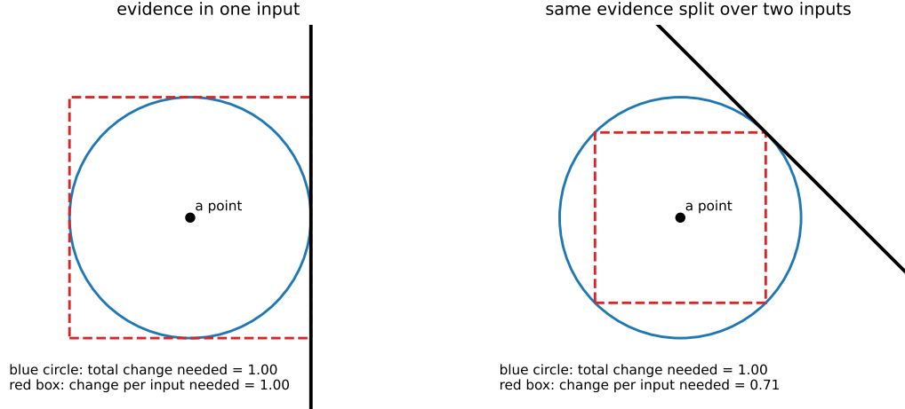
Figure 12: Two inputs, one point. Blue circle: total change needed to reach the decision boundary (black). Red dashed square: per-input change needed. Splitting the evidence over two inputs leaves the circle unchanged and shrinks the square.
