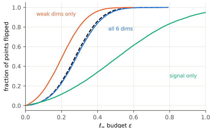
Figure 14: Share of test points flipped as the allowed nudge grows. The best possible rule (dashed black) lies on top of the trained network (blue). Networks that see only the five weak clues (orange) or only the reliable clue (green) are shown for comparison.
