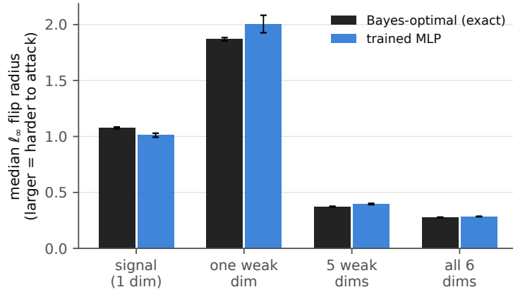
Figure 10: Median flip size (the smallest nudge that flips a point; larger means harder to attack) when the attacker controls only the listed inputs. Black: exact best rule. Blue: trained network (mean \pm s.d. over 10 runs).
