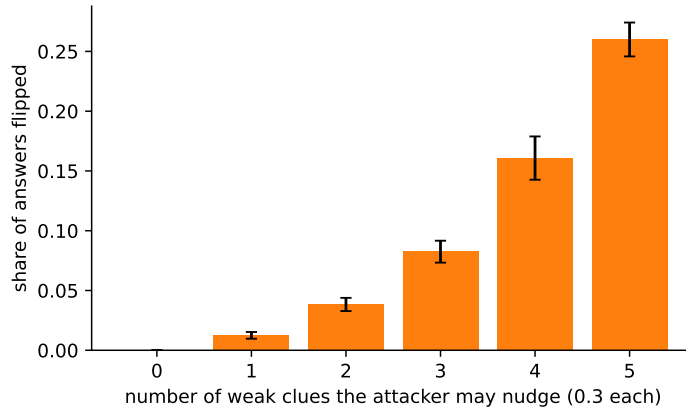
Figure 6: Share of answers flipped (Model A, nudge 0.3) as the attacker may nudge more and more of the weak clues. The reliable clue is never touched. Error bars: one standard deviation over 10 runs.
