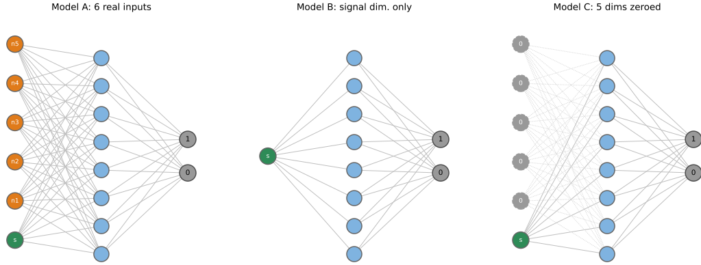
Figure 3: The three models. Green: the reliable clue. Orange: the weak clues (only A sees their values). Gray: slots that are always zero (C only).
