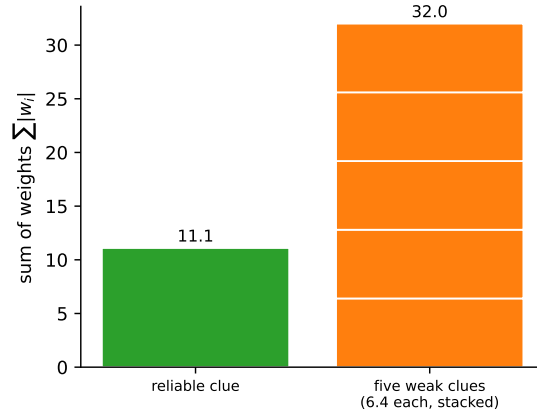
Figure 11: The sum of weights \sum |w_i| , which sets how far a full nudge moves the answer. One reliable clue carries 11.1; the five weak clues, stacked, carry 32.0.
