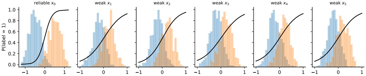
Figure 8: One training run. The network’s predicted probability of label 1 (black) as each input is varied alone (others held at their average), with the two classes’ distributions behind (blue: label 0, orange: label 1).
