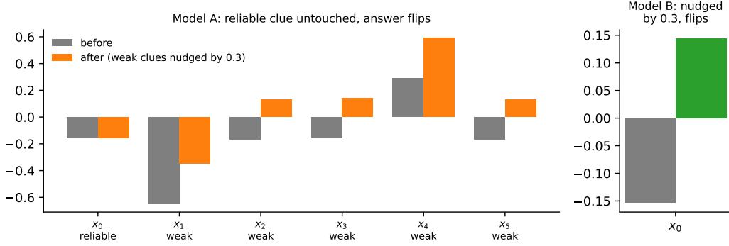
Figure 9: One successful attack per model at \epsilon = 0.3 on one test point, one training run. Left: attack allowed only on the weak clues; the reliable clue is unchanged yet the answer flips. Right: the model that sees only the reliable clue, attacked directly.
