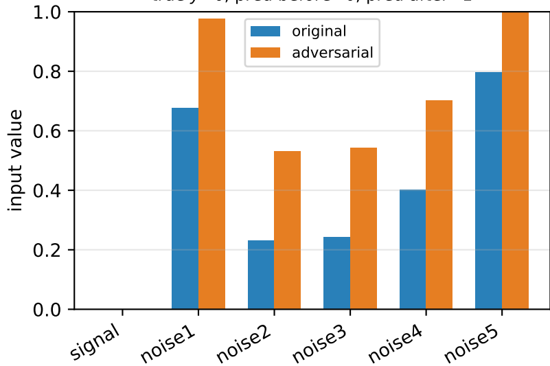
Model A, noise-only attack ( \epsilon=0.3 ) true y=0 , pred before=0, pred after=1
