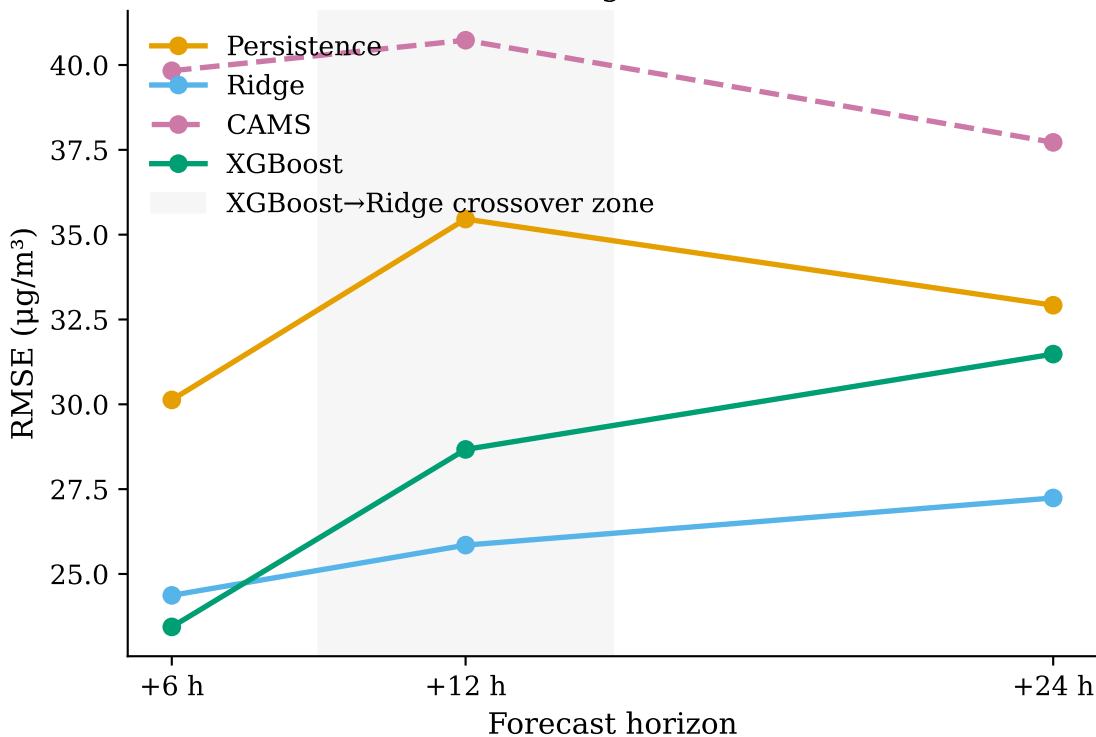
Figure 2. RMSE vs. forecast horizon — model ranking crossover (XGBoost leads at +6 h; Ridge leads at +12 h and +24 h)
