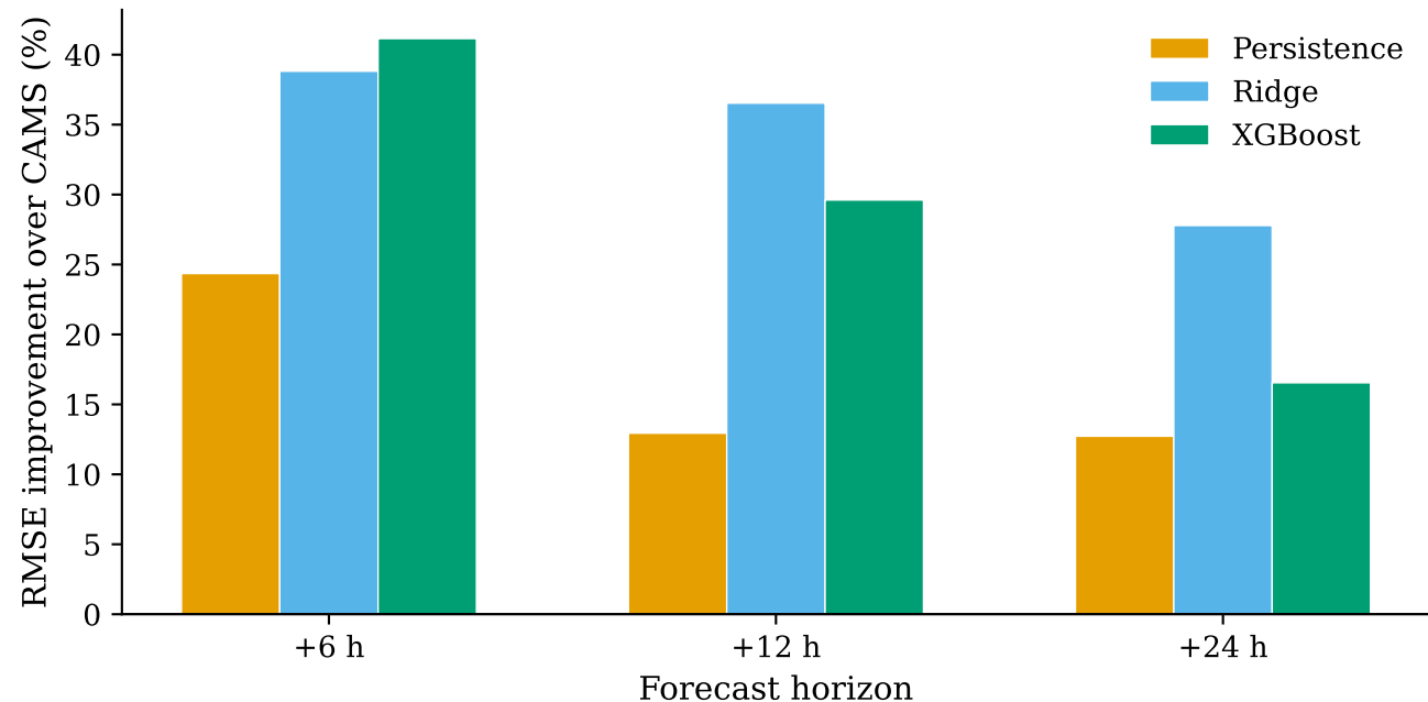
Figure 3. Relative RMSE improvement of local models over CAMS (positive = better than CAMS)
