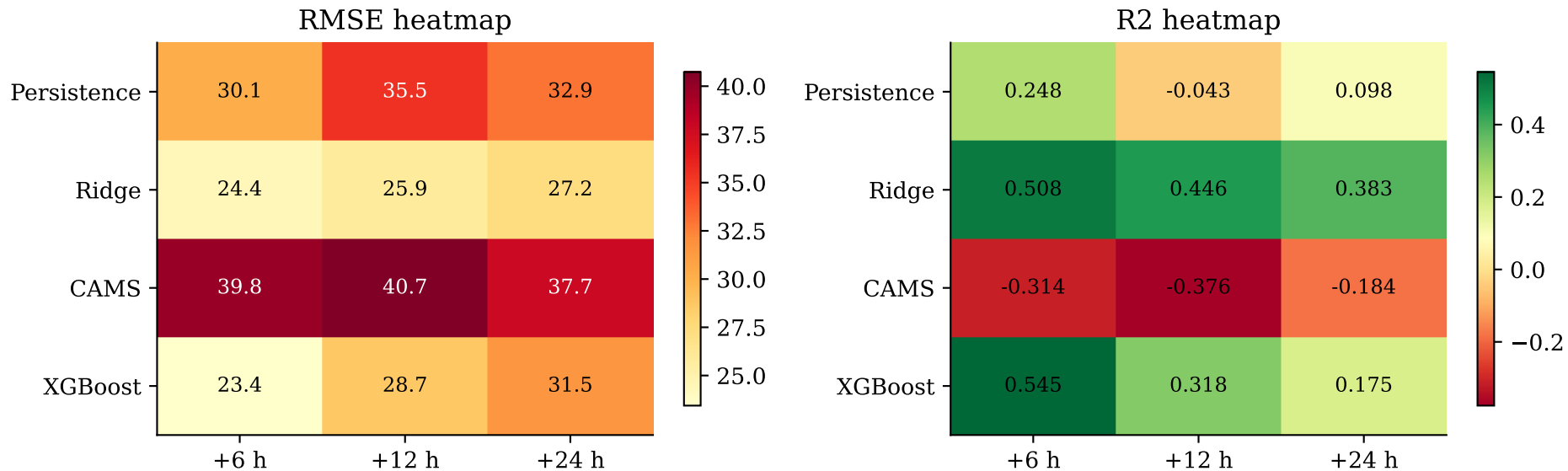
Figure 4. Full metric matrix — RMSE ( \mu\text{g}/\text{m}^3 ) and R^2 across all models and horizons
