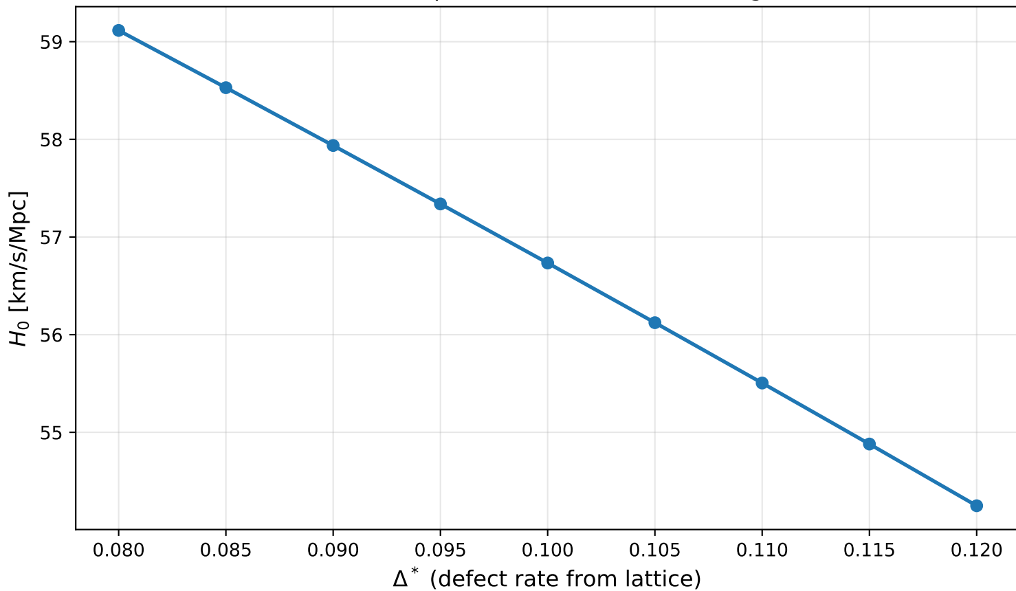
ICC-R2: H_0 dependence on \Delta^* ( \alpha=3.0 , \text{sign}=- )
