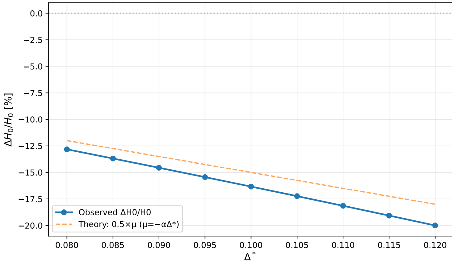
ICC-R2: Deviation from \Lambda CDM
